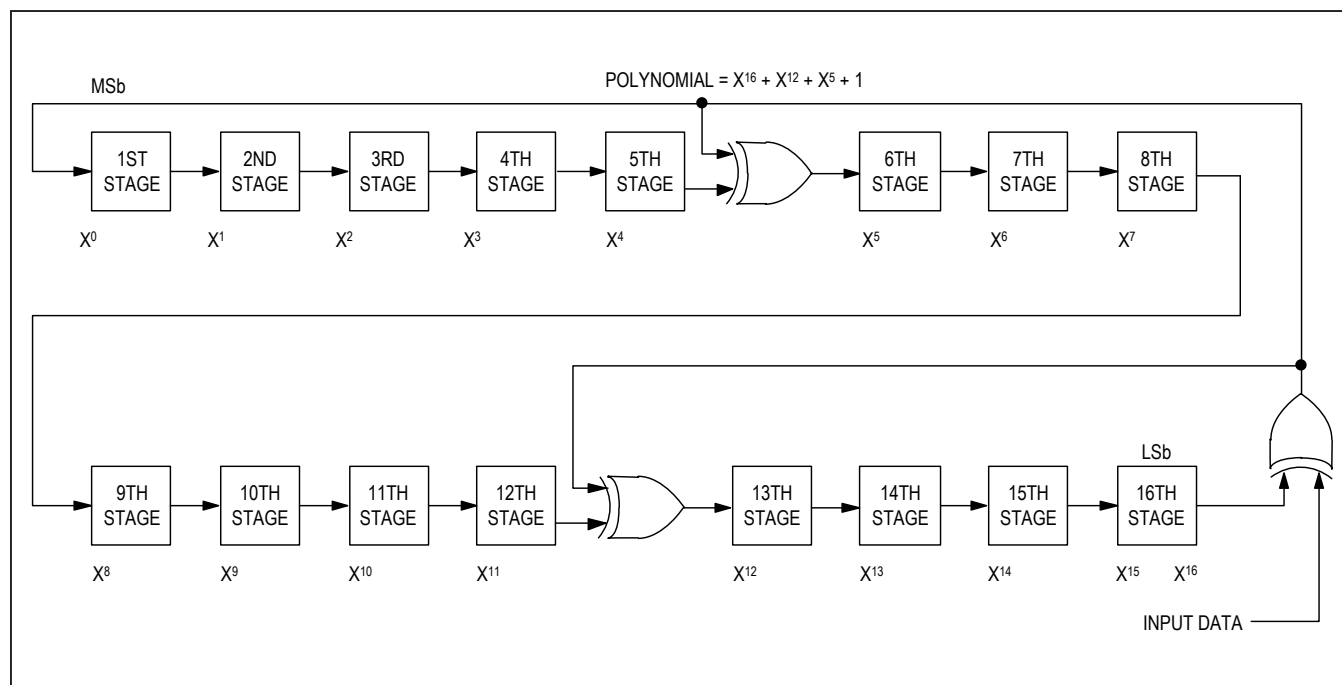
Figure 9. CRC-16-CCITT Generator
