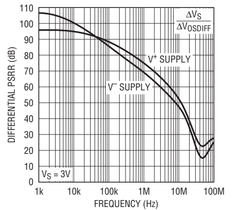
Differential Power Supply Rejection vs Frequency
