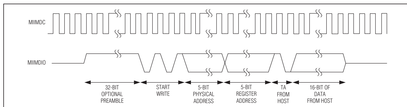
Figure 16. Write Behavior of the Management Data Unit
