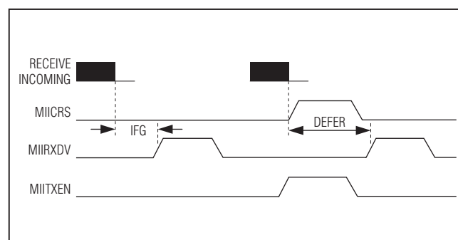
Figure 2. Receive Defer in MII Mode
