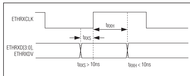
Figure 19. Receive Timing for Ethernet MAC Interface
