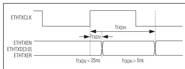
Figure 18. Transmit Timing for Ethernet MAC Interface
