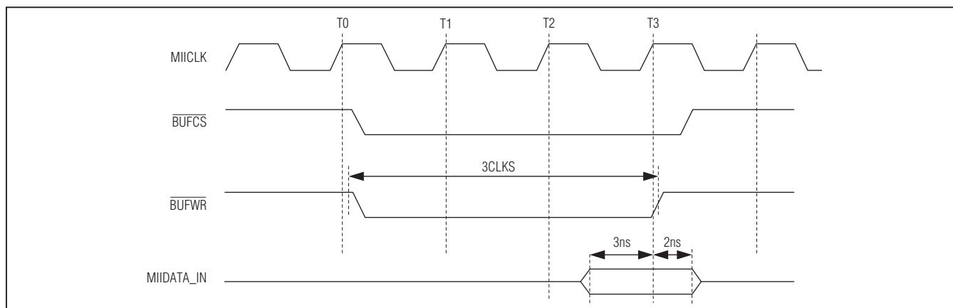
Figure 14. MAX2982 FIFO Write Timing Diagram
