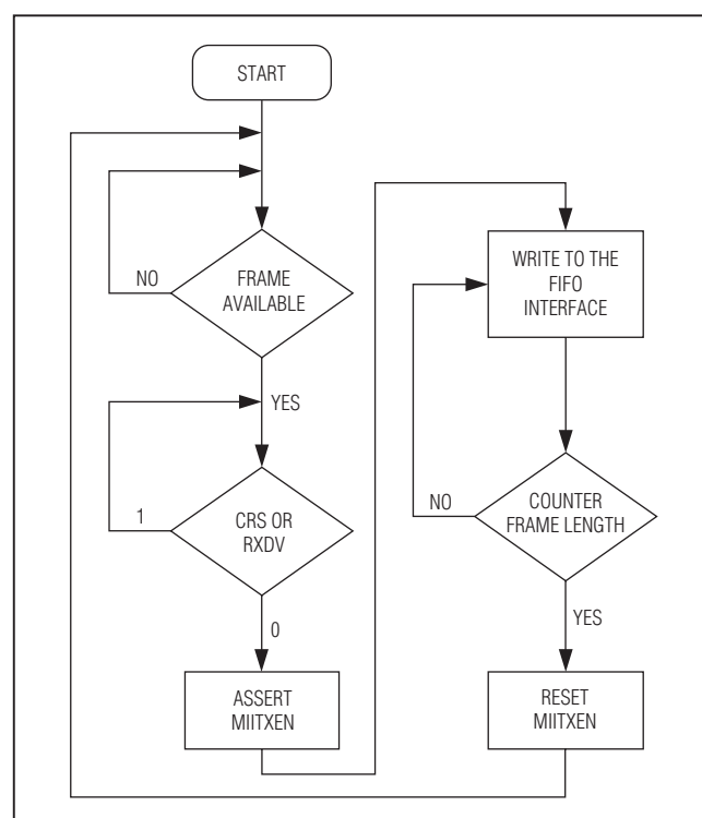
Figure 9. Buffering FIFO Transmission Process from External Host
