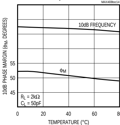
10dB PHASE MARGIN AND 10dB FREQUENCY vs. TEMP
