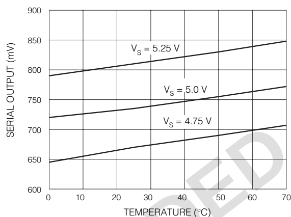
Fig. 4 Data and Data Output Voltage vs Temperature
