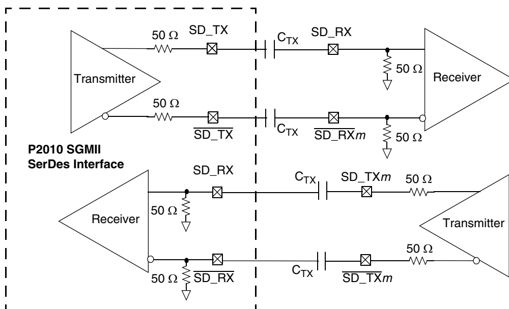
Figure 27. 4-Wire AC-Coupled SGMII Serial Link Connection Example
