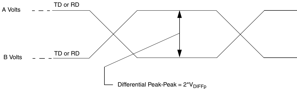
Figure 59. Differential Peak-Peak Voltage of Transmitter or Receiver
