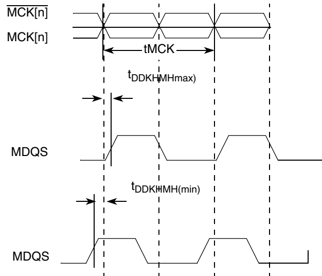
Figure 9. Timing Diagram for t_{\text{DDKMH}}
