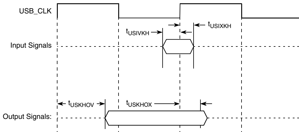
Figure 35. USB Signals
