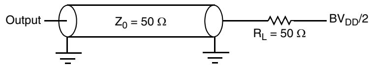
Figure 36. Enhanced Local Bus AC Test Load
