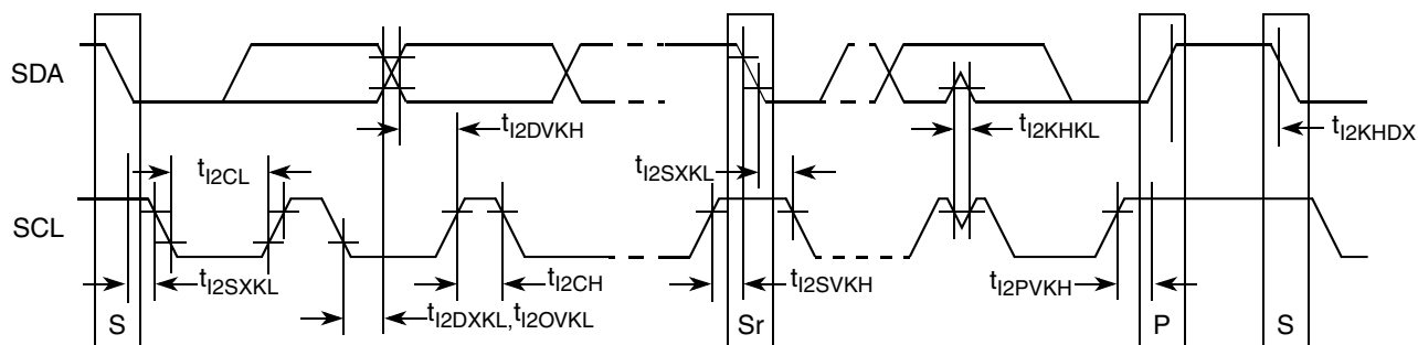
Figure 48. I 2 C Bus AC Timing Diagram
