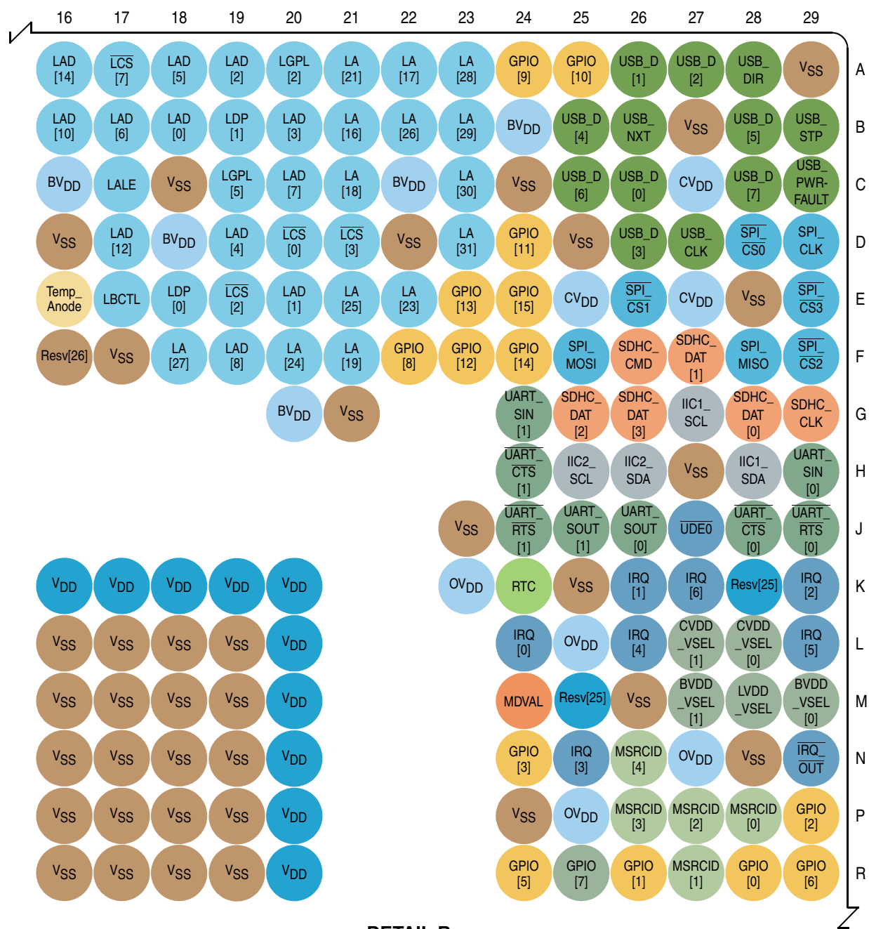
DETAIL B
