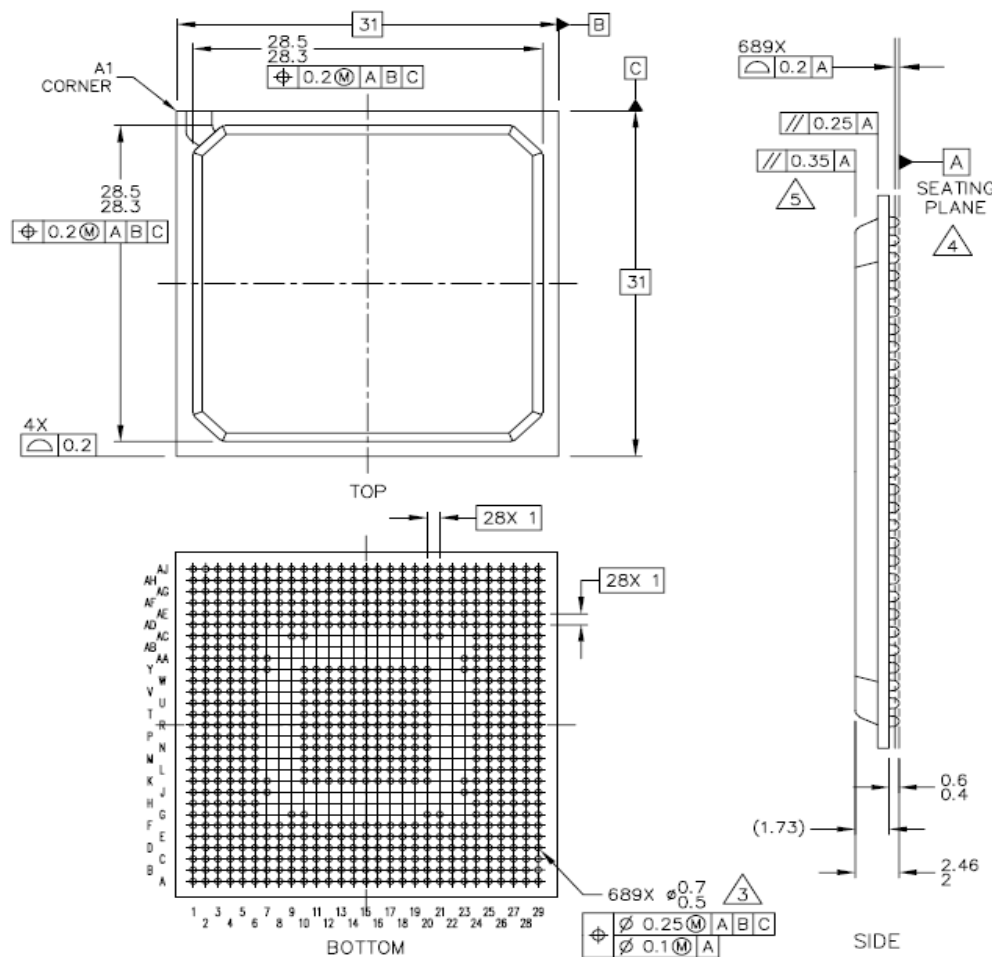
Figure 61. P2010 Package
