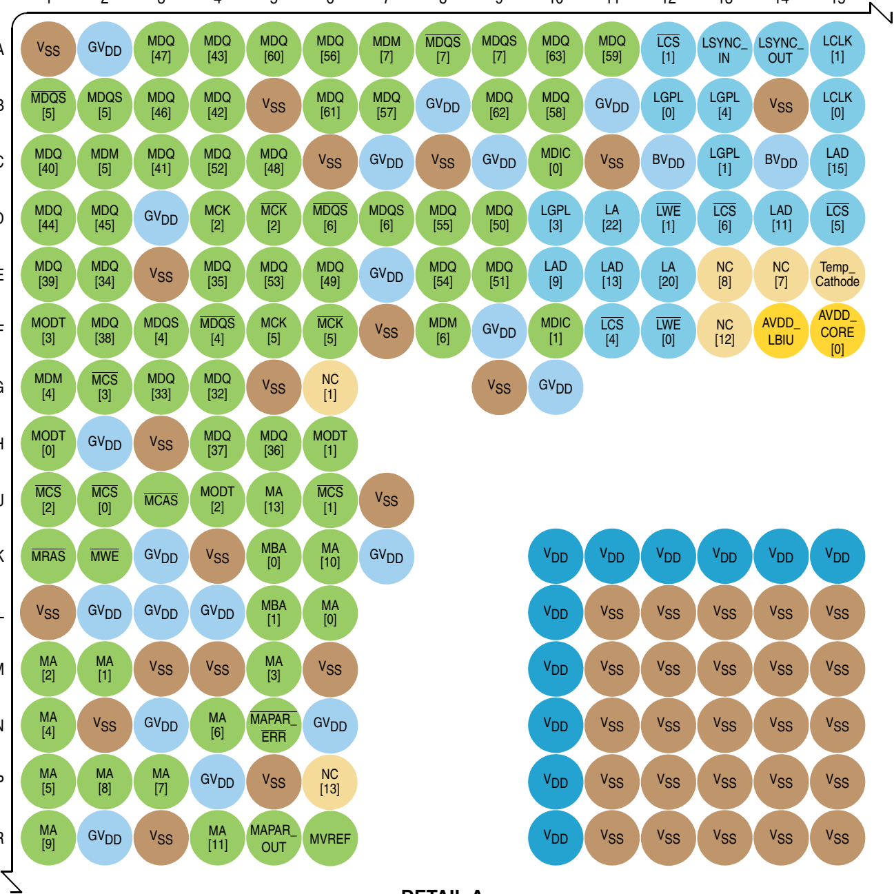
Figure 3. P2010 Ball Map—Detail A
