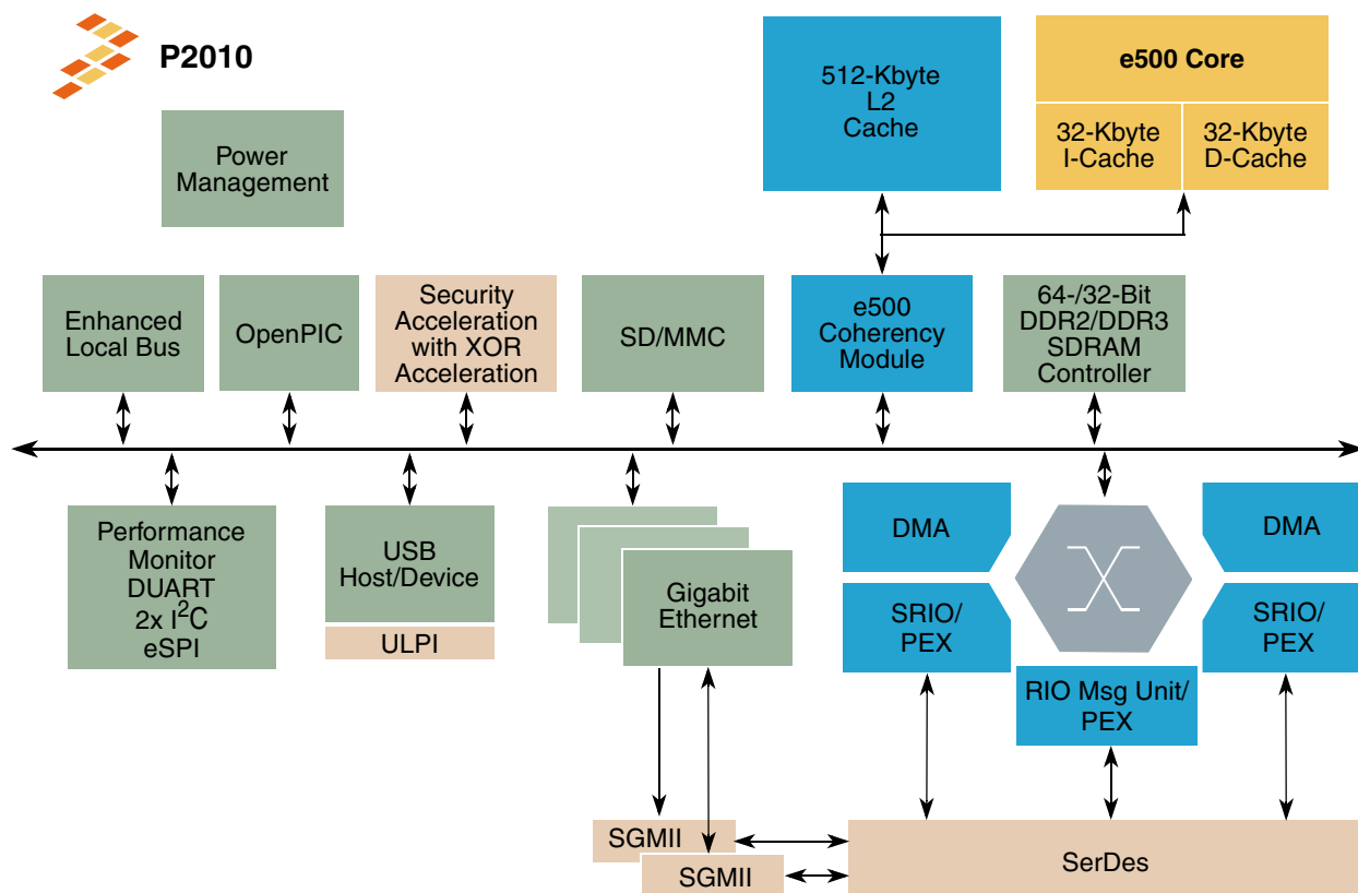
Figure 1. P2010 Block Diagram
