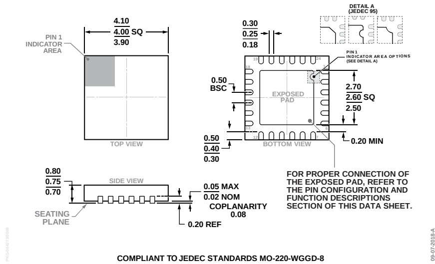
Figure 30. 24-Lead Lead Frame Chip Scale Package [LFCSP] 4 mm × 4 mm Body and 0.75 mm Package Height (CP-24-15) Dimensions shown in millimeters
