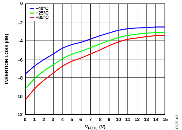
Figure 16. Minimum Insertion Loss vs. V_{\text{FCTL}} at Various Temperatures
