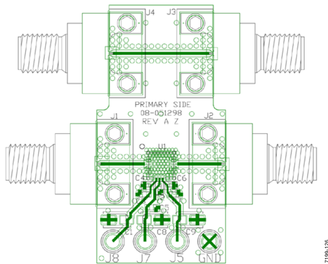
Figure 28. Evaluation PCB Layout, Top View
