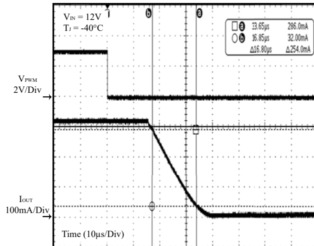
Figure 21 PWM Off
