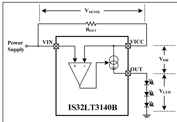
Figure 39 Voltage Drop
