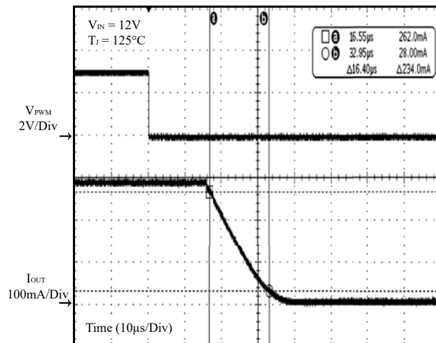
Figure 25 PWM Off
