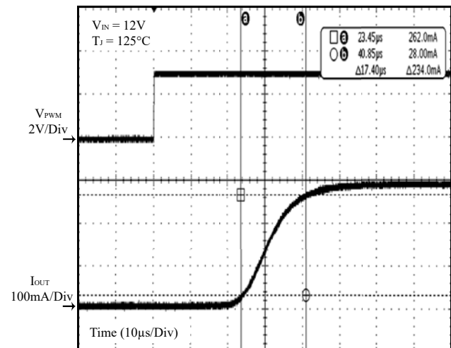
Figure 26 PWM On
