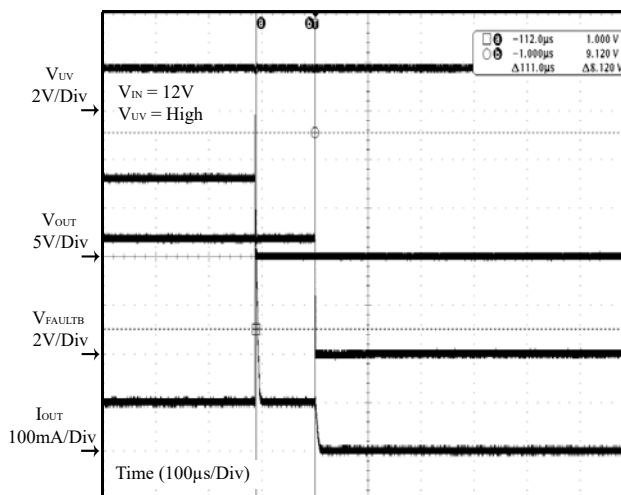
Figure 34 Output Short
