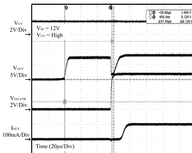
Figure 36 Output Short Fault Remove
