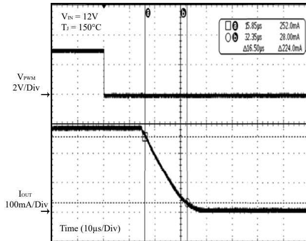
Figure 27 PWM Off
