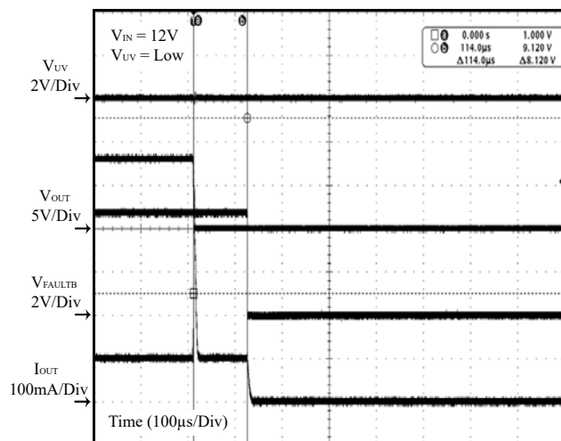
Figure 33 Output Short
