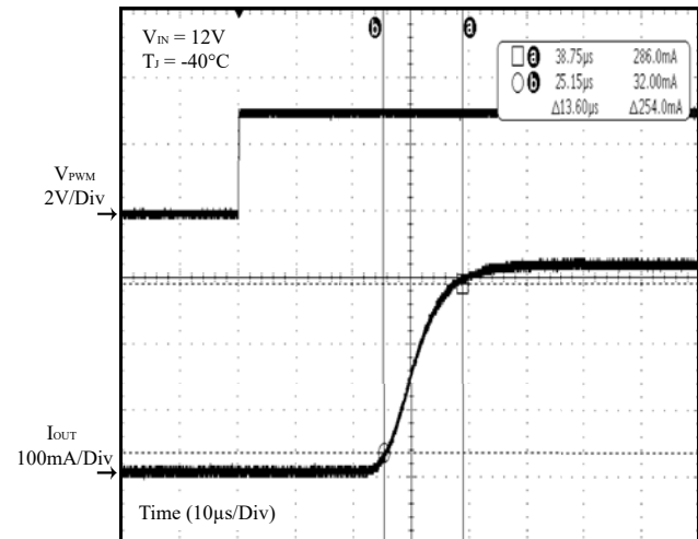
Figure 22 PWM On
