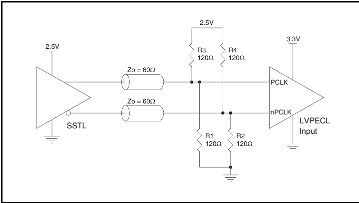
Figure 2D. PCLK/nPCLK Input Driven by a 3.3V SSTL Driver
