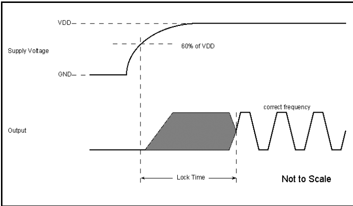
Lock Time
