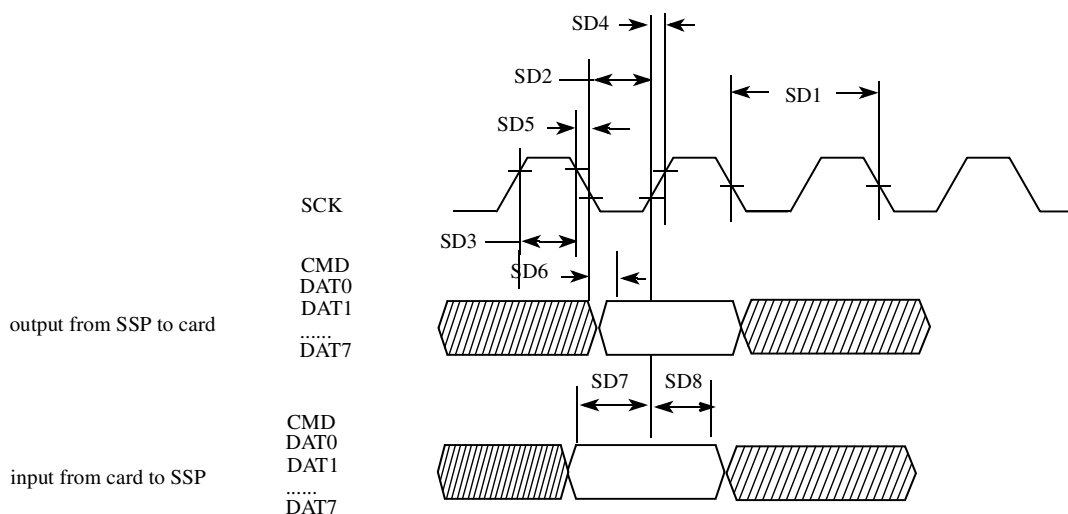
Figure 36. SD/MMC4.3 Timing
