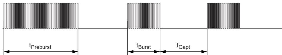
Figure 4-2. IR Signal
