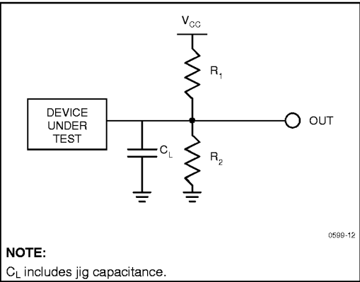
Figure 13. Test Configuration
