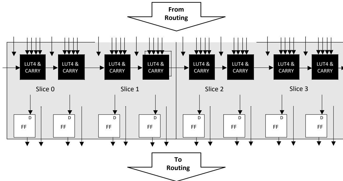
Figure 2.2. PFU Diagram
