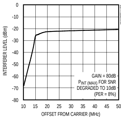
RECEIVER BLOCKER REJECTION vs. CARRIER OFFSET
