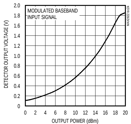
PA POWER-DETECTOR OUTPUT VOLTAGE vs. OUTPUT POWER
