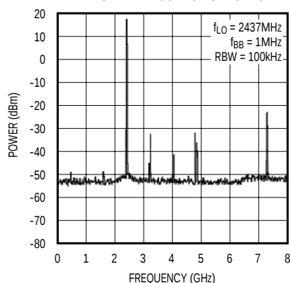
TRANSMITTER OUTPUT SPECTRUM
