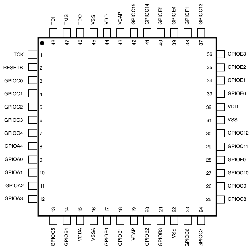
Figure 23. 48-pin LQFP
