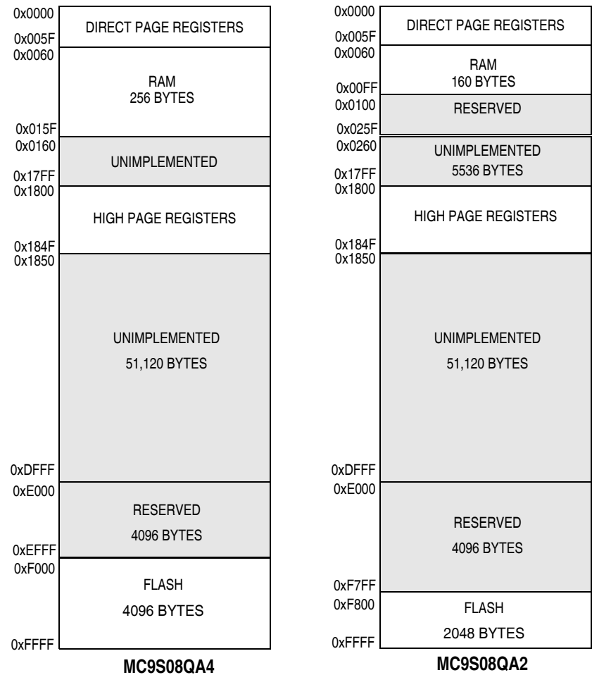
Figure 4-1. MC9S08QA4 Series Memory Map
