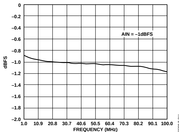
Figure 14. Gain Flatness
