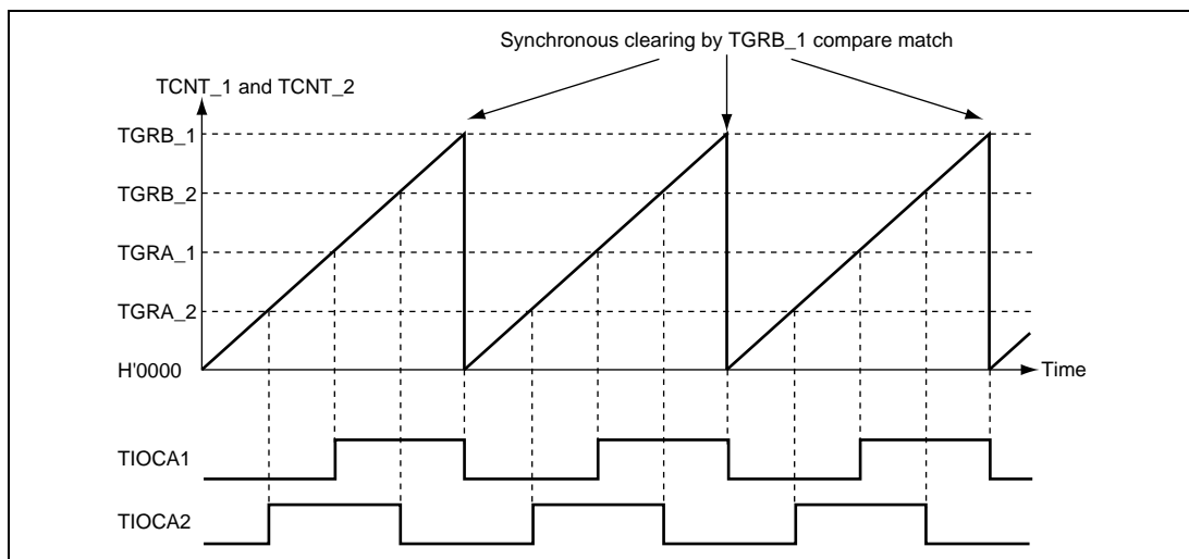
Figure 12.14 Example of Synchronous Operation
