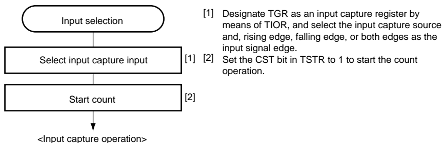
Figure 12.11 Example of Setting Procedure for Input Capture Operation
