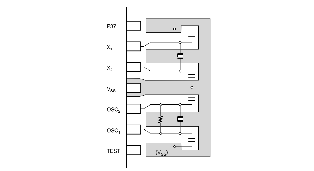
Figure 5.9 Example of Crystal and Ceramic Resonator Arrangement
