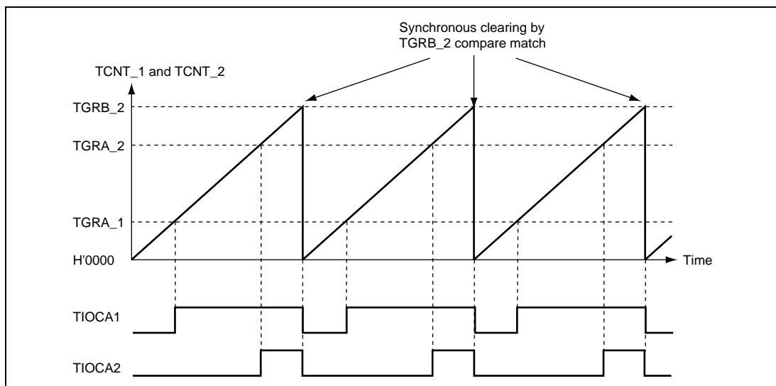
Figure 12.19 Example of PWM Mode Operation (2)
