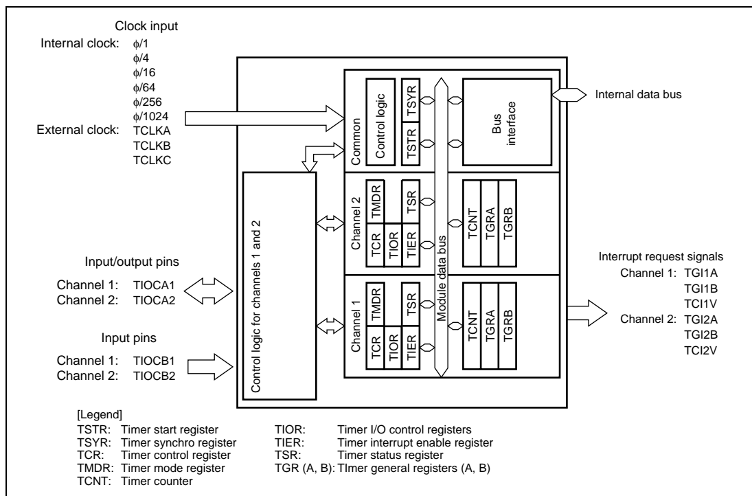
Figure 12.1 Block Diagram of TPU
