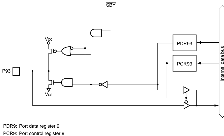
Figure B.8 (a) Port 9 Block Diagram (P93)
