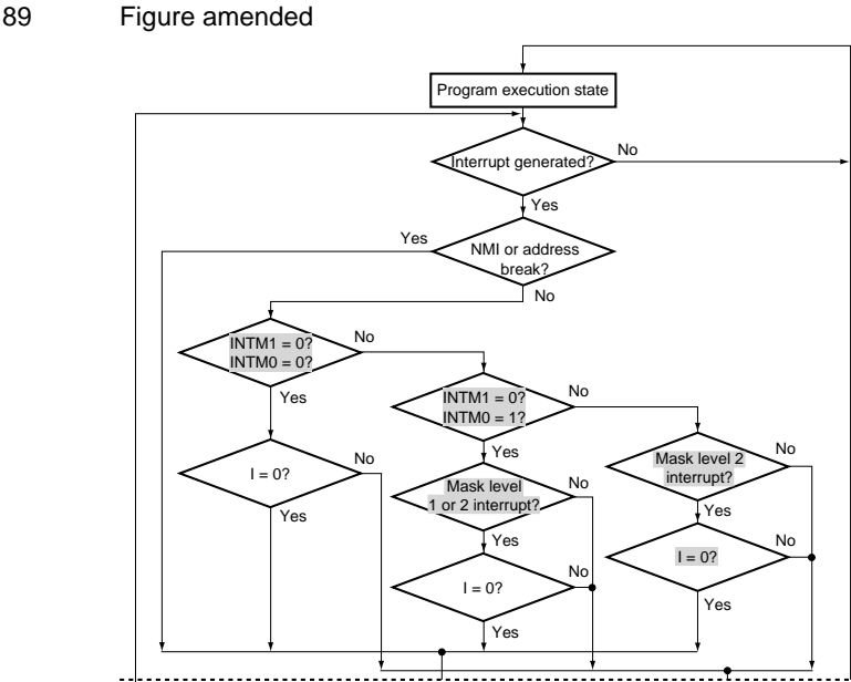
Figure 4.2 Flowchart of Procedure Up to Interrupt Acceptance
