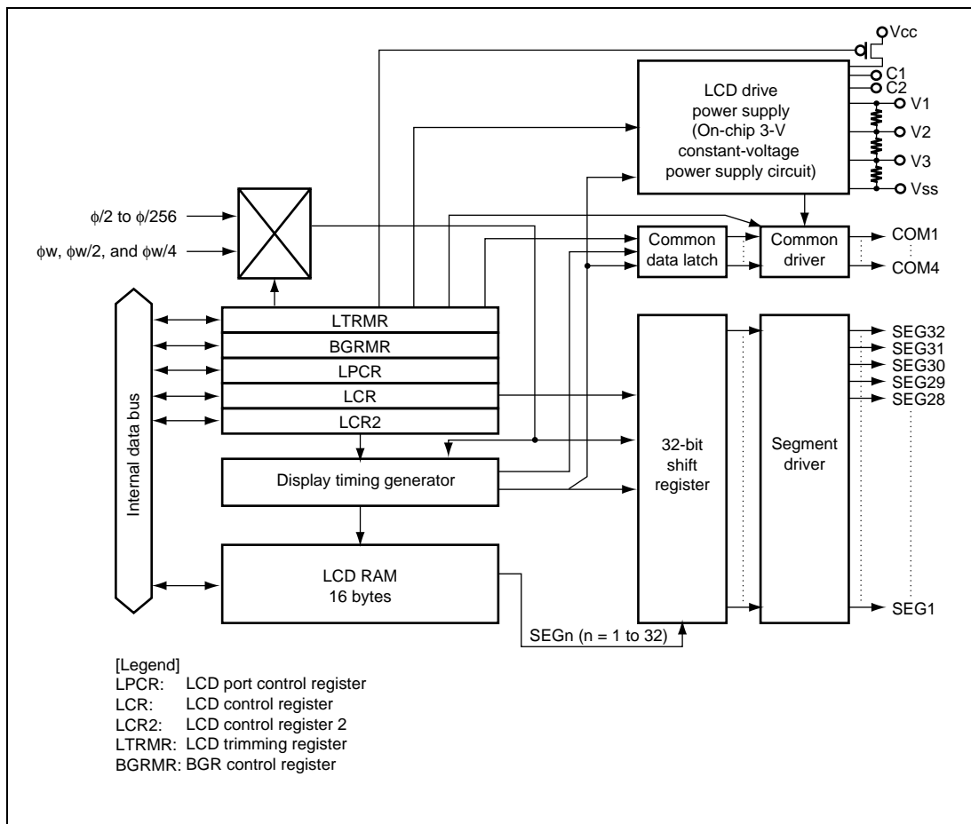
Figure 19.1 Block Diagram of LCD Controller/Driver
