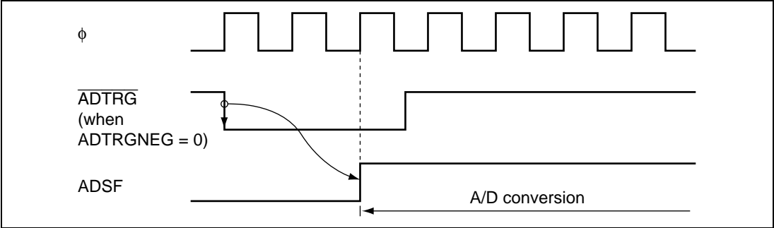
Figure 18.2 External Trigger Input Timing
