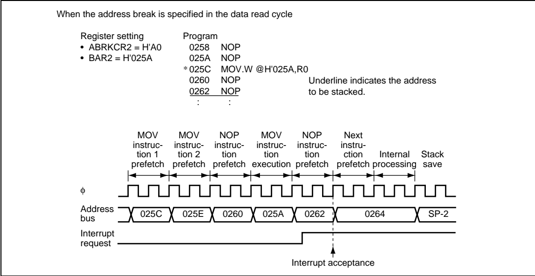
Figure 22.2 Address Break Interrupt Operation Example (2)
