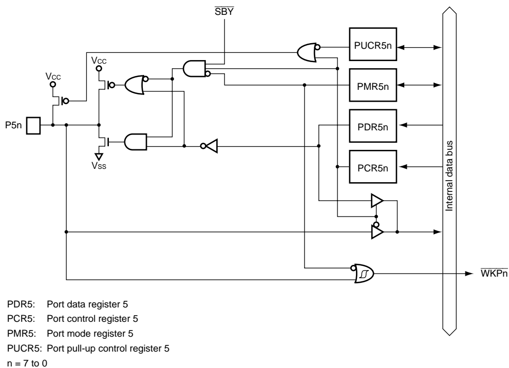
Figure B.4 Port 5 Block Diagram
