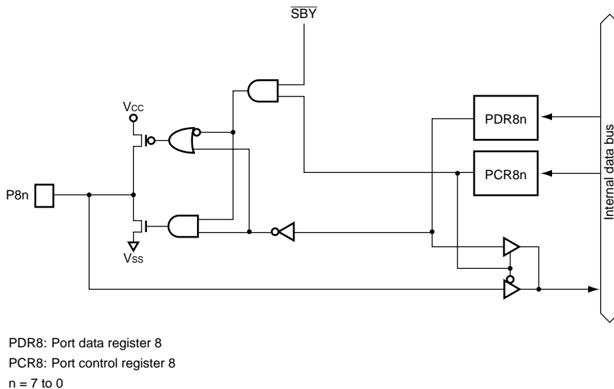
Figure B.7 Port 8 Block Diagram
