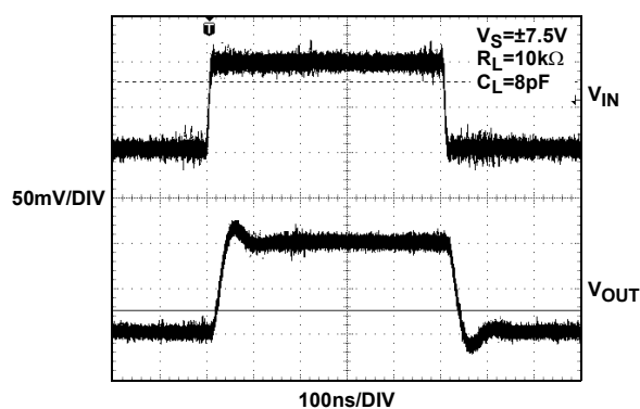
FIGURE 12. SMALL SIGNAL TRANSIENT RESPONSE ( V_{COM} )
