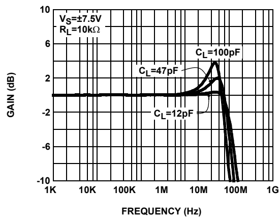
FIGURE 2. FREQUENCY RESPONSE FOR VARIOUS C_{LOAD} (BUFFER)
