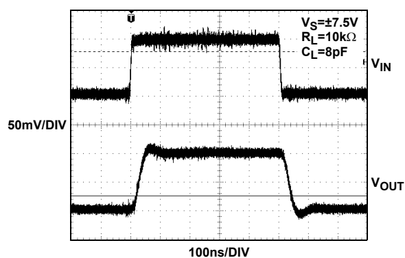
FIGURE 4. SMALL SIGNAL TRANSIENT RESPONSE (BUFFER)
