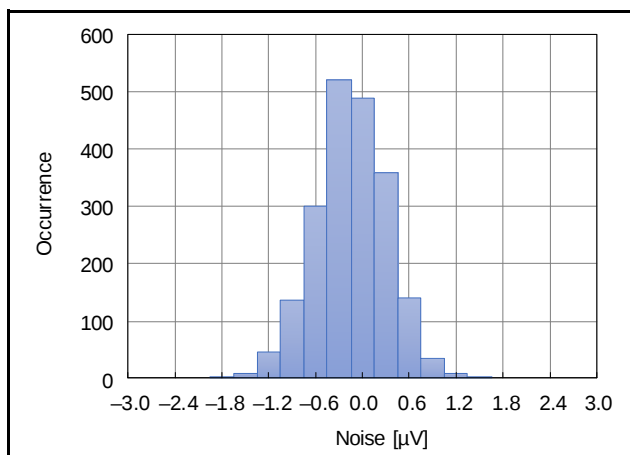
Figure 2.85 Noise Histogram (AVCC0 = 5.0 V, T_a = 25°C, Low Power Mode, Gain = 1 (PGA disabled, BUF disabled), f_{DR} = 1.9 SPS, V_{ID} = 0V, V_{REF} = 2.5V)
