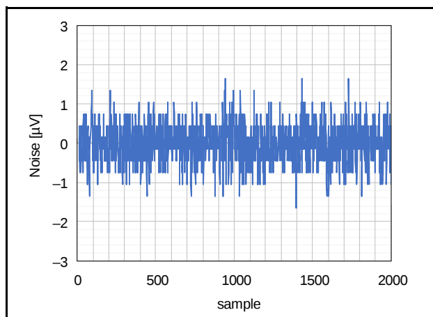
Figure 2.86 Plot of Noise (AVCC0 = 5.0 V, T_a = 25°C, Low Power Mode, Gain = 1 (PGA disabled, BUF disabled), f_{DR} = 1.9 SPS, V_{ID} = 0V, V_{REF} = 2.5V)
