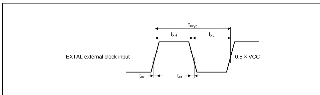
Figure 2.36 EXTAL External Clock Input Timing
