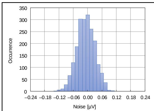
Figure 2.81 Noise Histogram (AVCC0 = 5.0 V, T_a = 25°C, Low Power Mode, Gain = 128, f_{DR} = 1.9 SPS, V_{ID} = 0V, V_{REF} = 2.5V)
