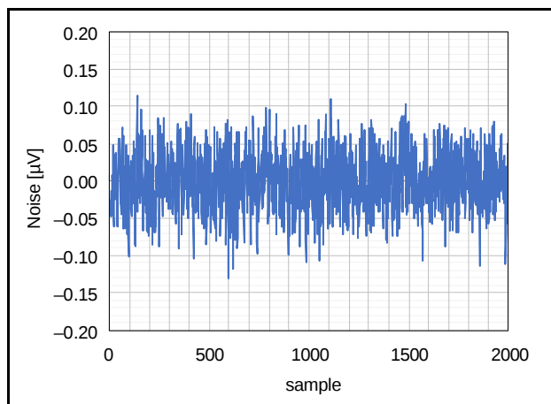
Figure 2.82 Plot of Noise (AVCC0 = 5.0 V, T_a = 25°C, Low Power Mode, Gain = 128, f_{DR} = 1.9 SPS, V_{ID} = 0V, V_{REF} = 2.5V)
