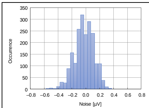
Figure 2.83 Noise Histogram (AVCC0 = 5.0 V, T_a = 25°C, Low Power Mode, Gain = 16, f_{DR} = 1.9 SPS, V_{ID} = 0V, V_{REF} = 2.5V)
