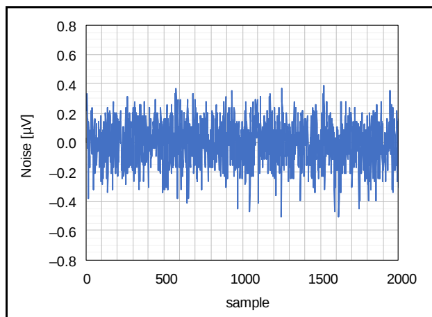
Figure 2.84 Plot of Noise (AVCC0 = 5.0 V, T_a = 25°C, Low Power Mode, Gain = 16, f_{DR} = 1.9 SPS, V_{ID} = 0V, V_{REF} = 2.5V)
