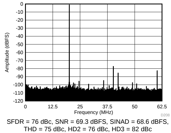
Figure 98. FFT for 270-MHz Input Signal (Dither Off)
