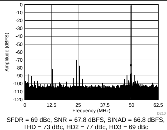
Figure 100. FFT for 450-MHz Input Signal (Dither Off)
