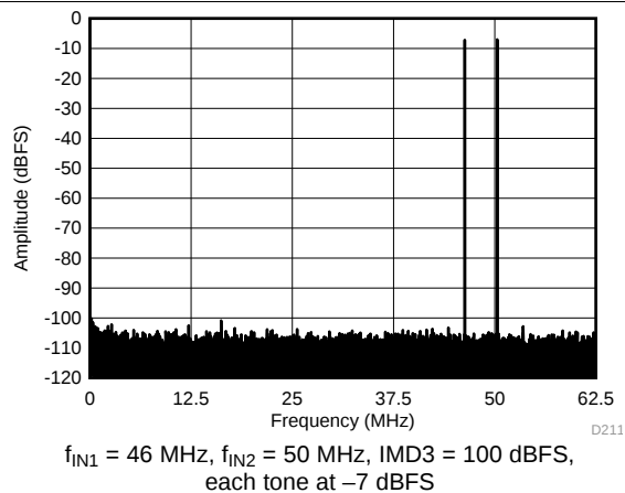
Figure 101. FFT for Two-Tone Input Signal ( -7\text{ dBFS} at 46 MHz and 50 MHz)
