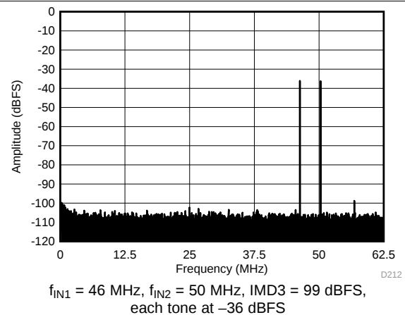
Figure 102. FFT for Two-Tone Input Signal ( -36\text{ dBFS} at 46 MHz and 50 MHz)
