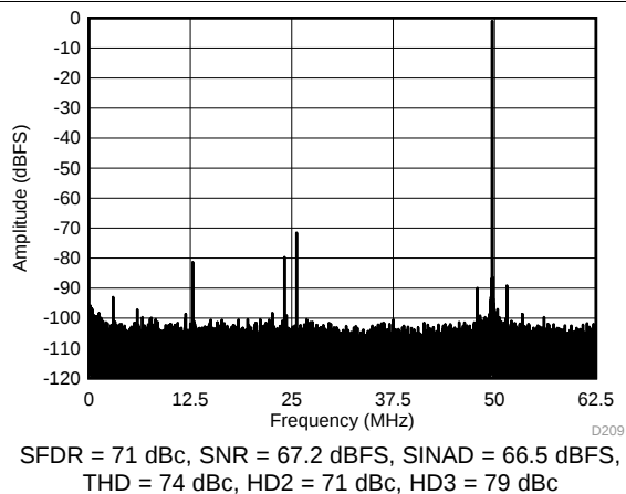
Figure 99. FFT for 450-MHz Input Signal (Dither On)
