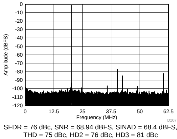
Figure 97. FFT for 270-MHz Input Signal (Dither On)
