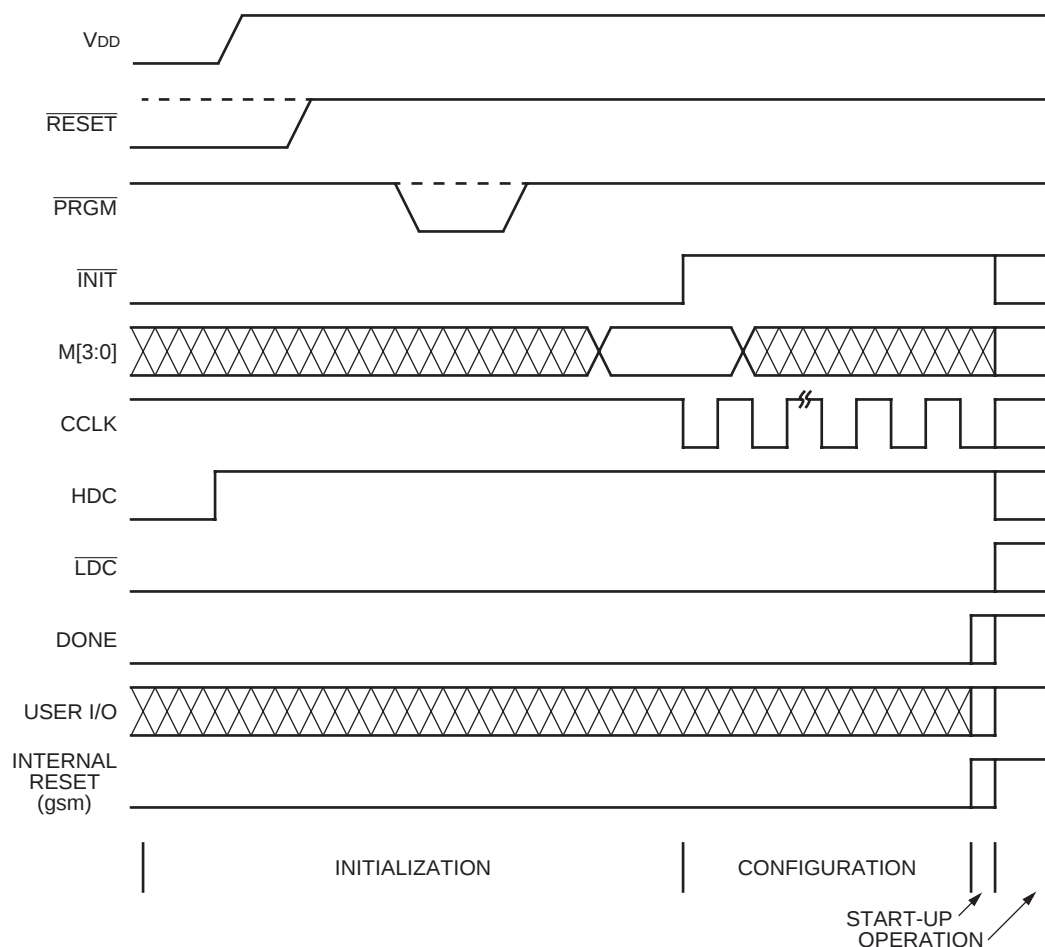
Figure 37. Initialization/Configuration/Start-Up Waveforms
