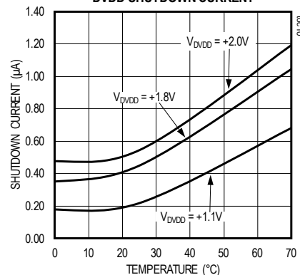
DVDD SHUTDOWN CURRENT
