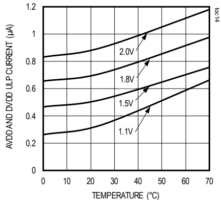
AVDD AND DVDD ULP CURRENT vs. TEMPERATURE
