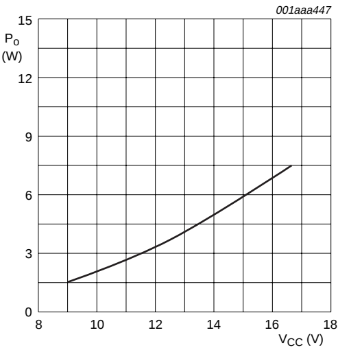
Fig 8. Output power as function of supply voltage.
