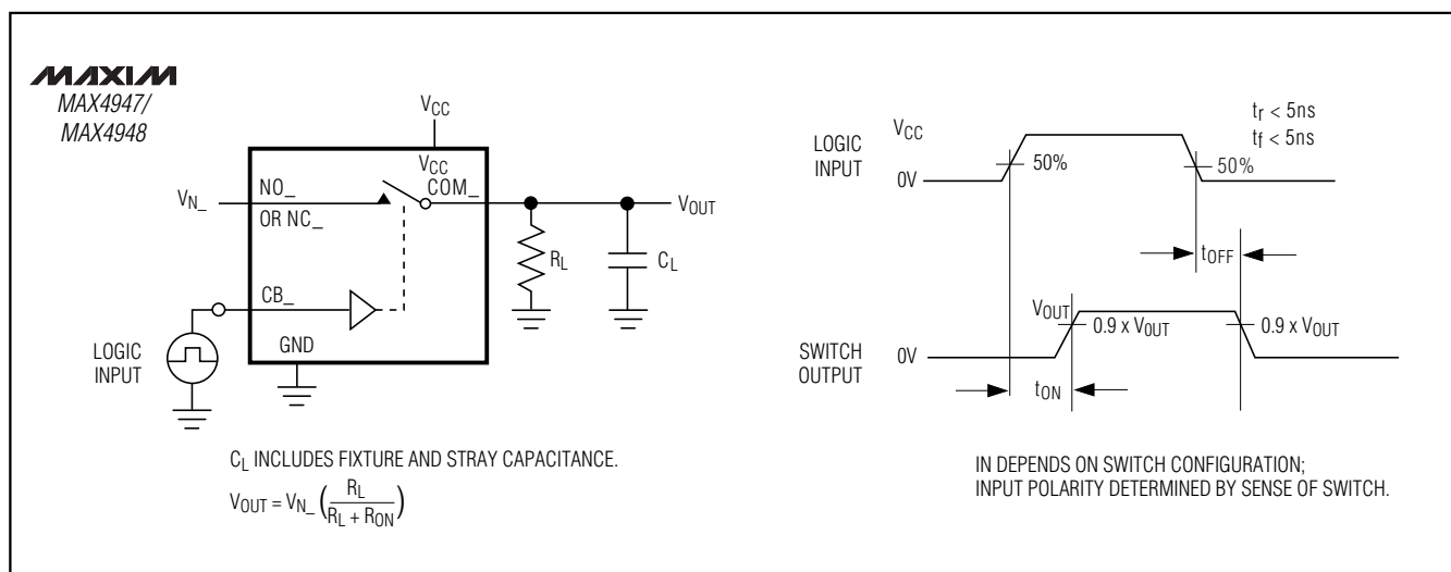
Figure 1. Switching Time
