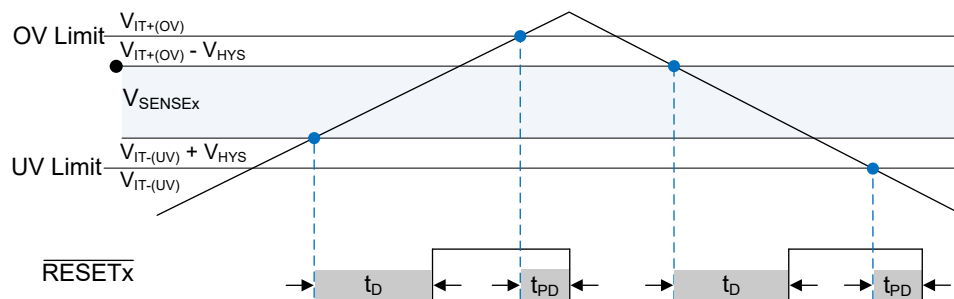
Figure 8-6. \overline{\text{RESETx}} Output
