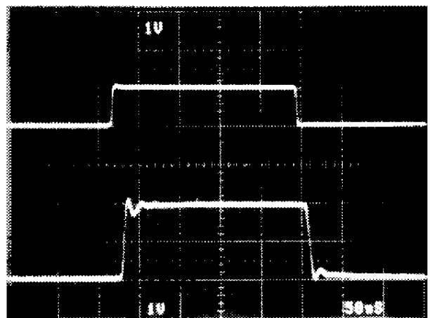
FIGURE 6. LARGE SIGNAL RESPONSE
