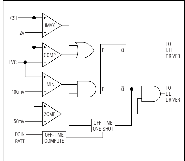
Figure 9. DC-DC Converter Block Diagram
