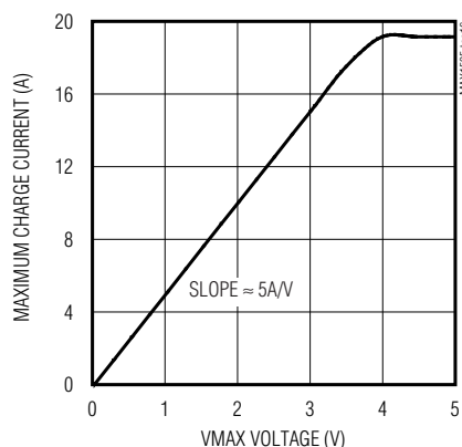
MAXIMUM CHARGE CURRENT vs. V_{MAX}
