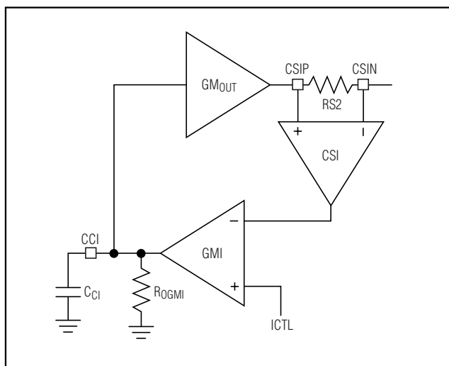
Figure 12. CCI Loop Diagram
