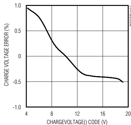
CHARGE-VOLTAGE ACCURACY
