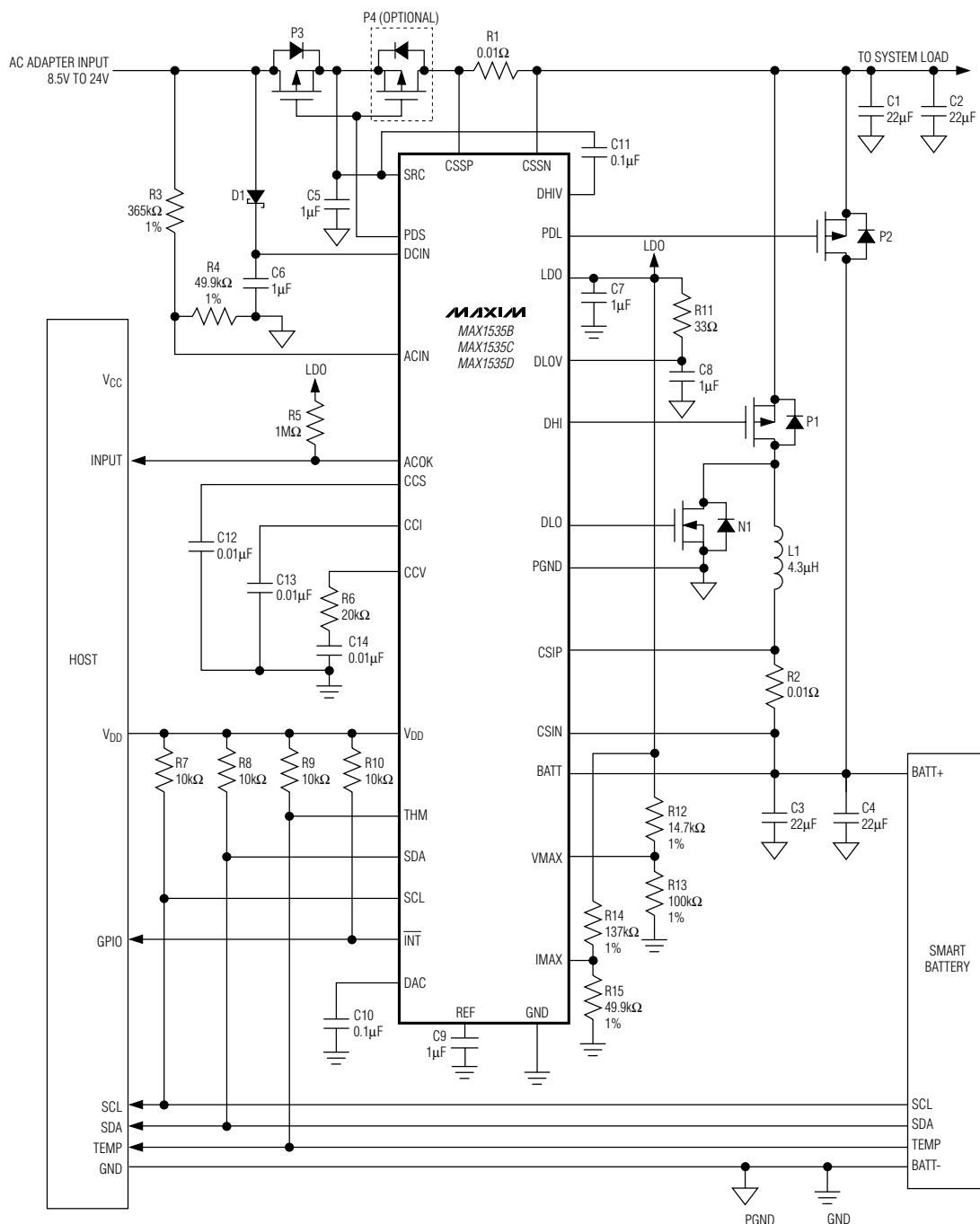
Figure 1. Standard Application Circuit
