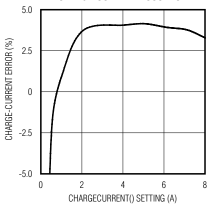
CHARGE-CURRENT ACCURACY
