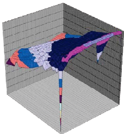
Figure 35. BUCK MINI Efficiency C_0 = 1\mu\text{F} , \text{ESR} = 1\Omega , L = 33\mu\text{F} Automatic Mode
