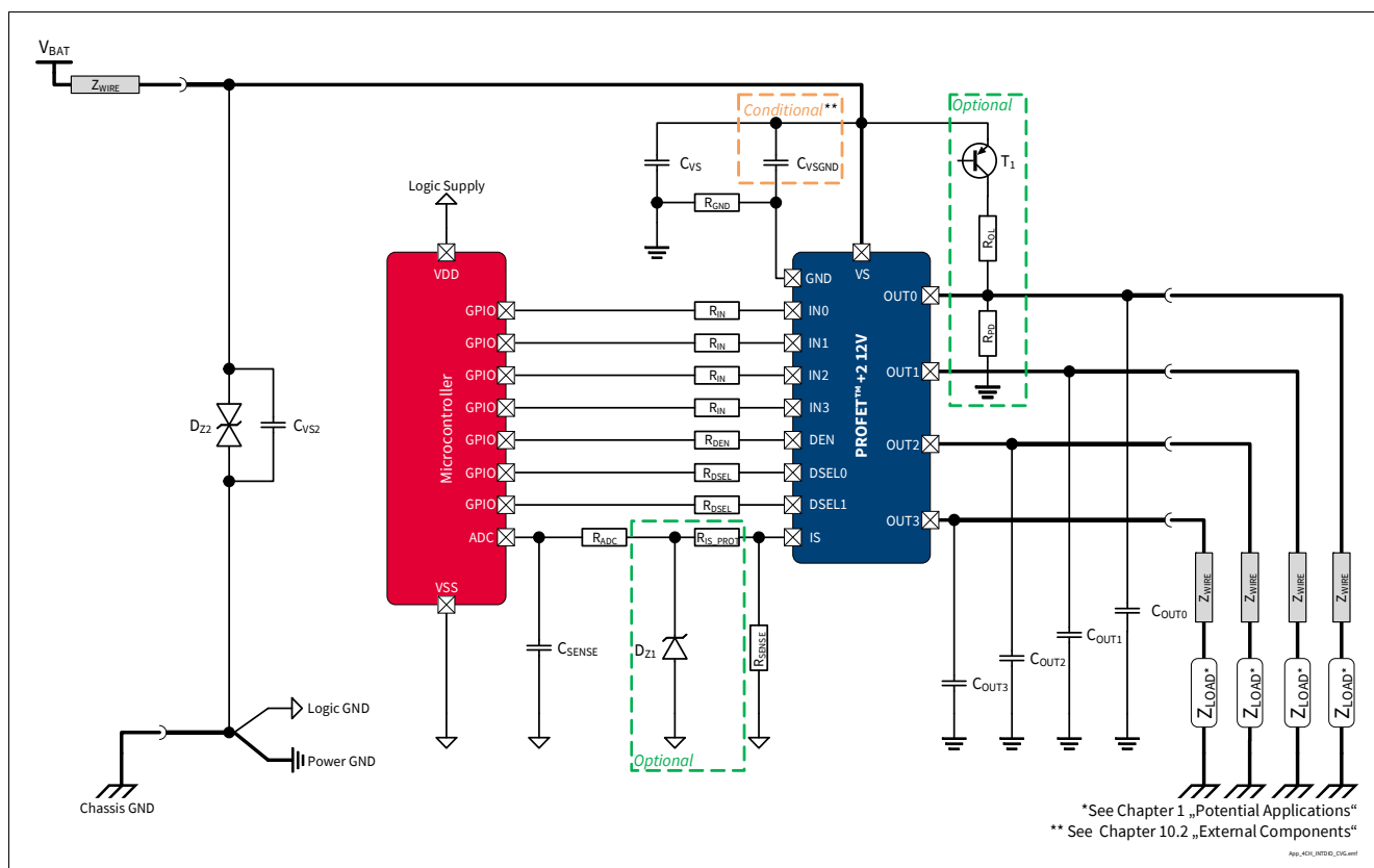
Figure 42 BTS7200-4EPA Application Diagram
