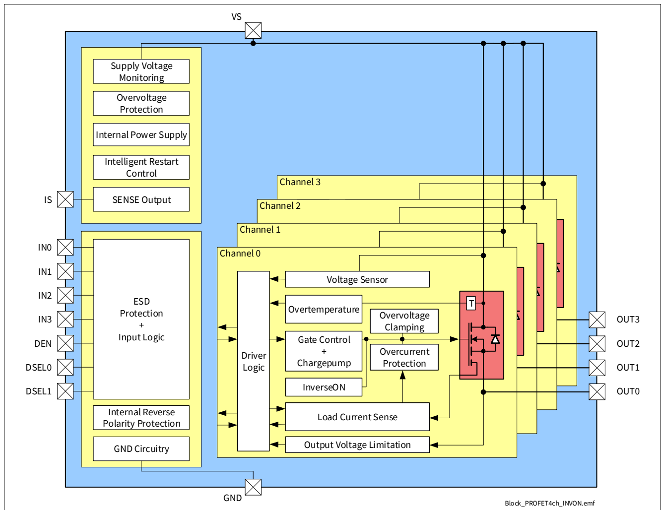
Figure 2 Block Diagram of BTS7200-4EPA
