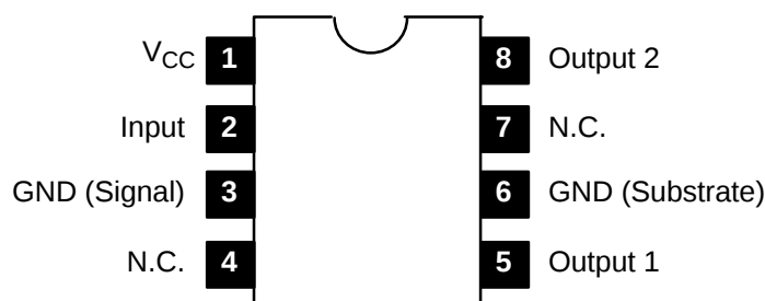
Pin Connection Diagram
