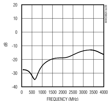
S11
