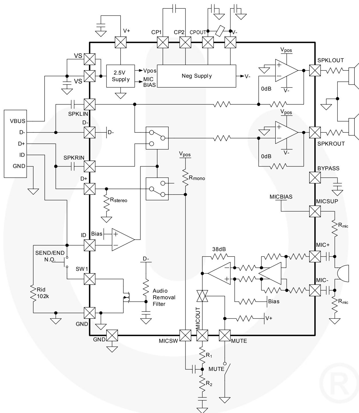
Figure 2. Block Diagram
