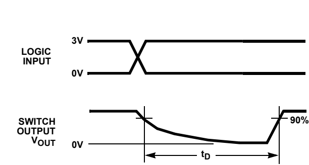
FIGURE 2C. MEASUREMENT POINTS (ISL84544 ONLY)
