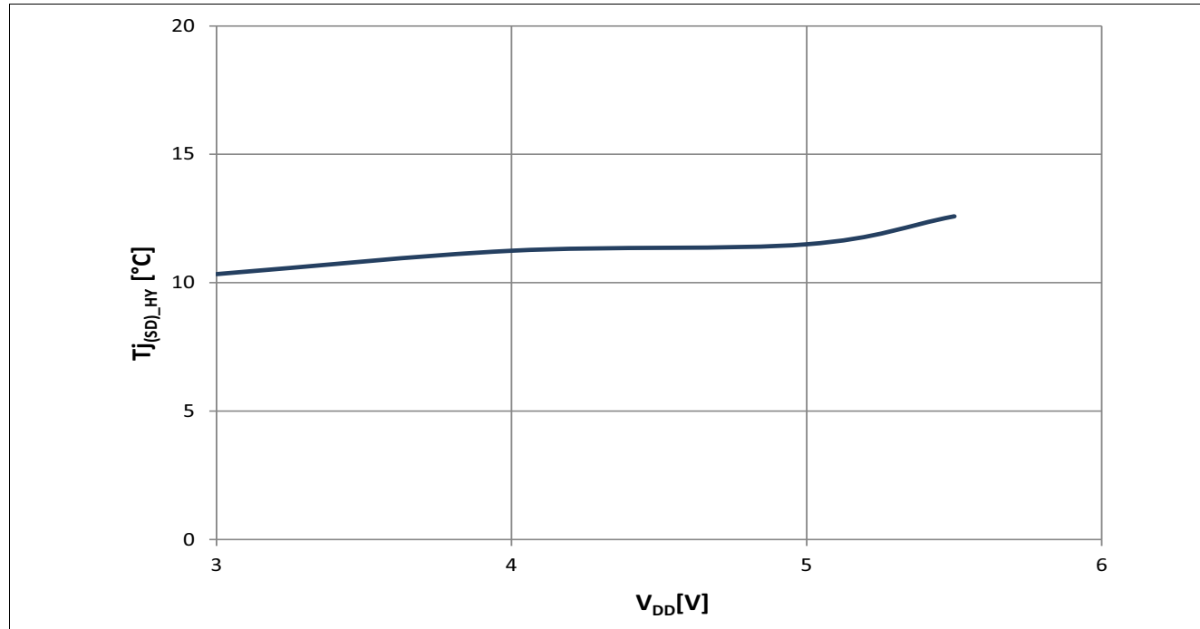
Figure 42 Typical T j(sd)_HYS vs V DD @ I L =10mA
