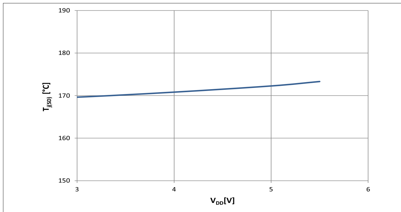
Figure 41 Typical T j(sd) vs V DD @ I L =10mA
