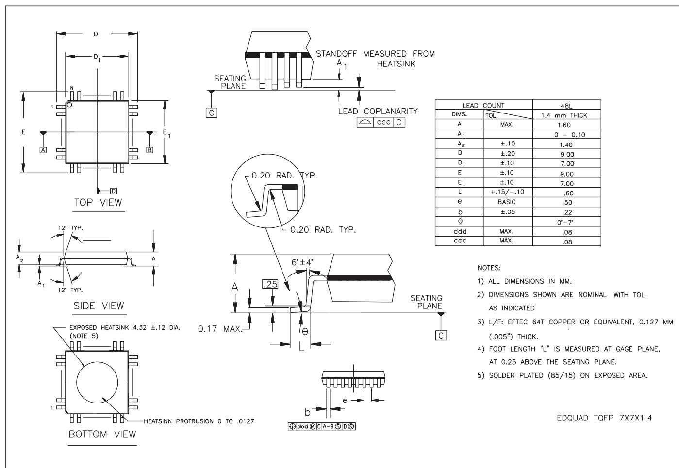
Figure 7. Package 48 Lead TQFP, Power Enhanced
