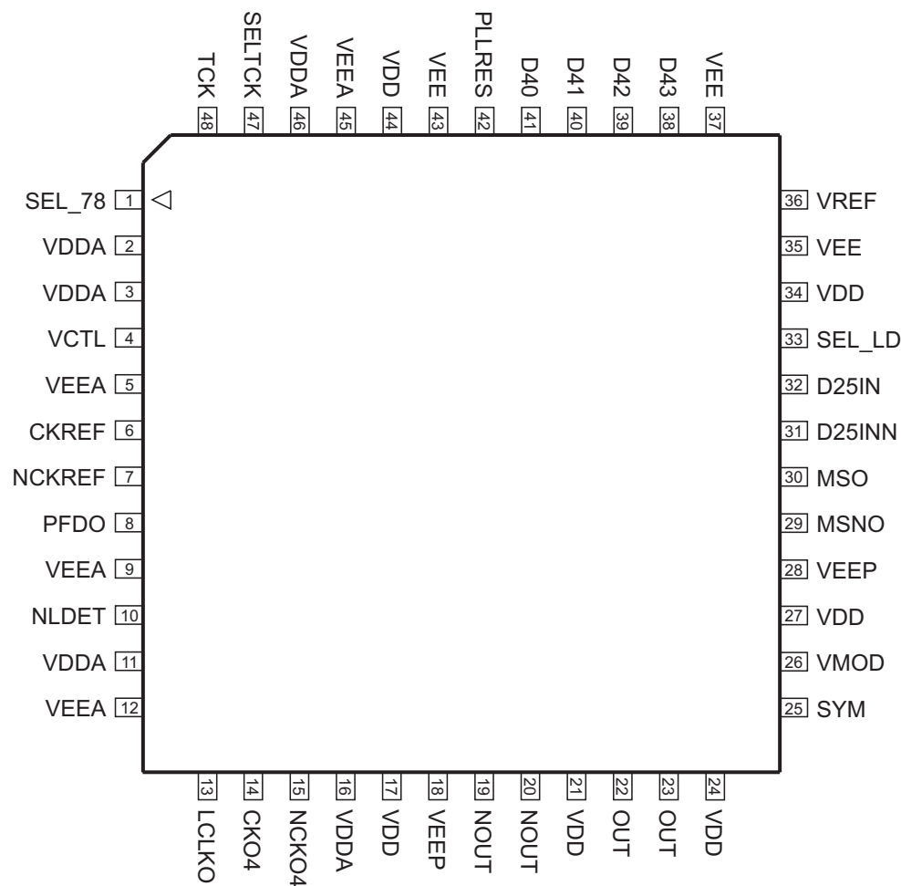
Figure 6. Package Pinout, 48 Lead TQFP - Top View
