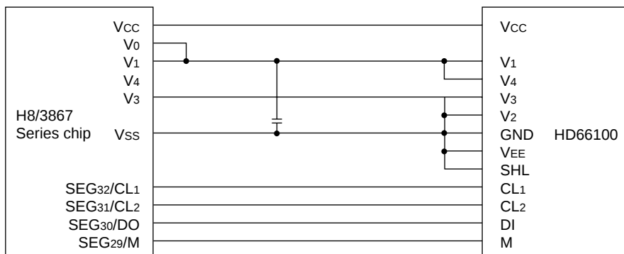
Figure 13.18 Connection to HD66100
