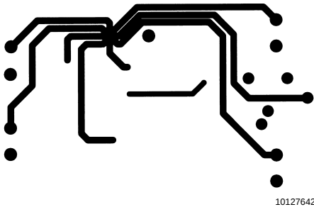
Recommended SOP PC Board Layout: Bottom Layer
