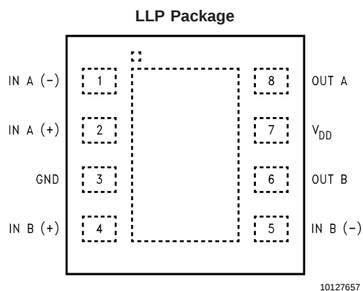
Top View Order Number LM4808LD See NS Package Number LDA08B
