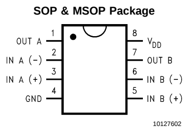
Top View Order Number LM4808M, LM4808MM See NS Package Number M08A, MUA08A
