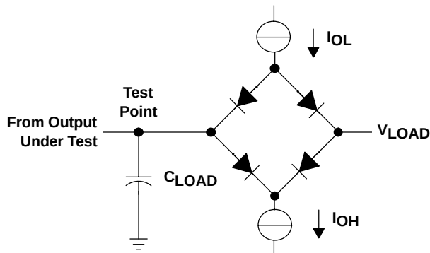
LOAD CIRCUIT
