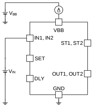
Figure 25. Operating Current
