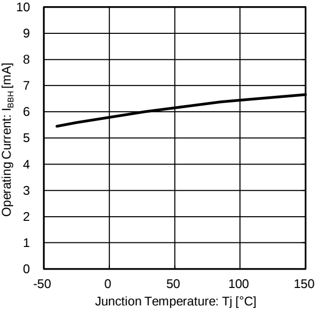
Figure 9. Operating Current vs Junction Temperature
