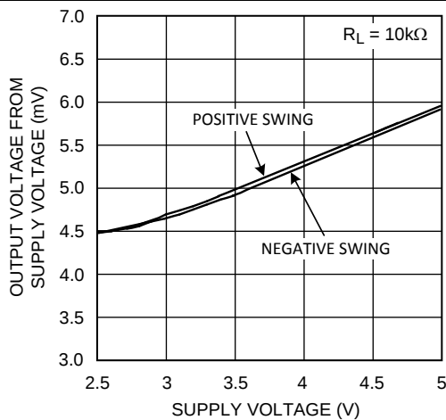
Figure 4. Output Voltage Swing vs Supply Voltage
