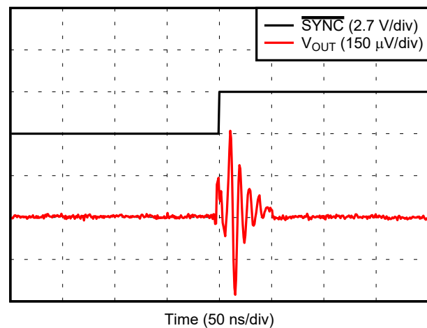
Figure 6-24. Control Feedthrough
