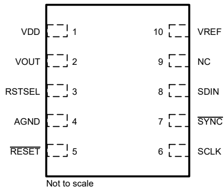
Figure 5-1. DRX (10-Pin WSON) Package, Top View
