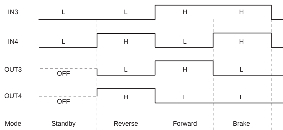
(2) Constant current channel timing chart
