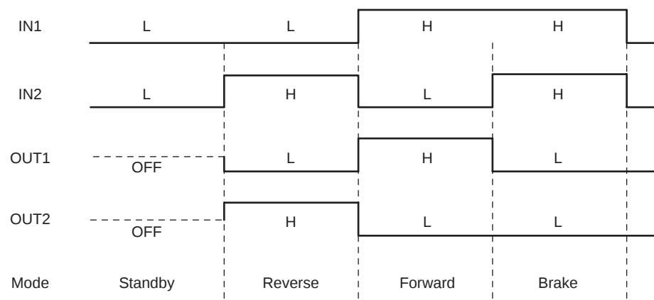
(1) Constant voltage channel timing chart
