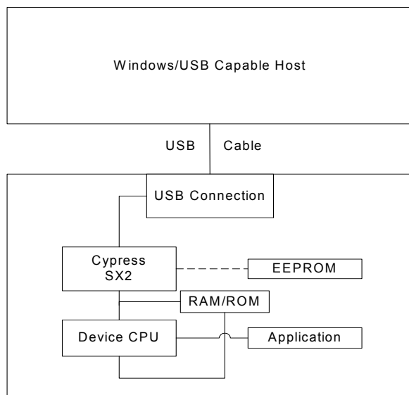
Figure 4-1. Example USB System Diagram
