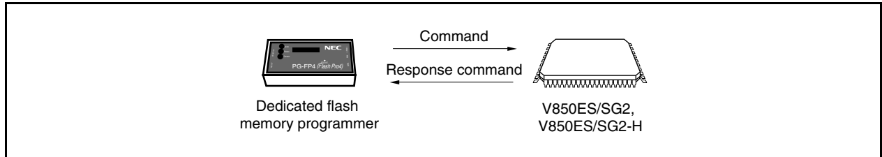
Figure 30-10. Communication Commands
