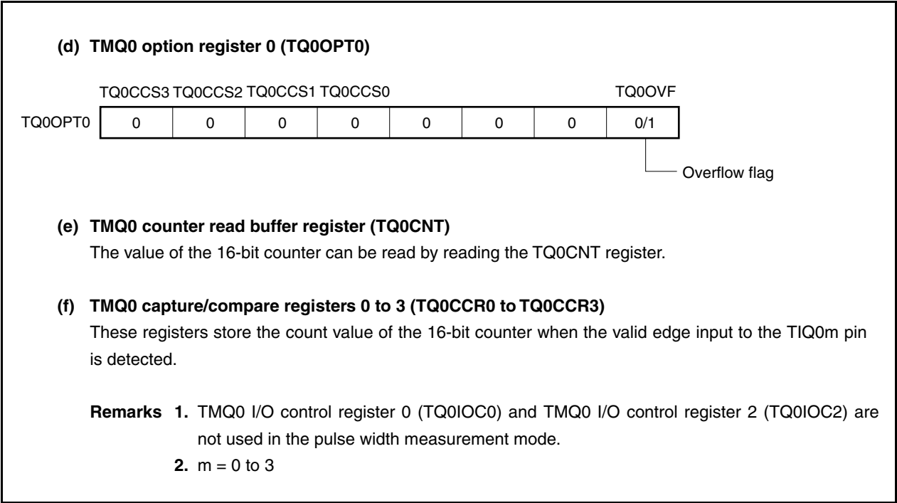
Figure 8-40. Register Setting in Pulse Width Measurement Mode (2/2)
