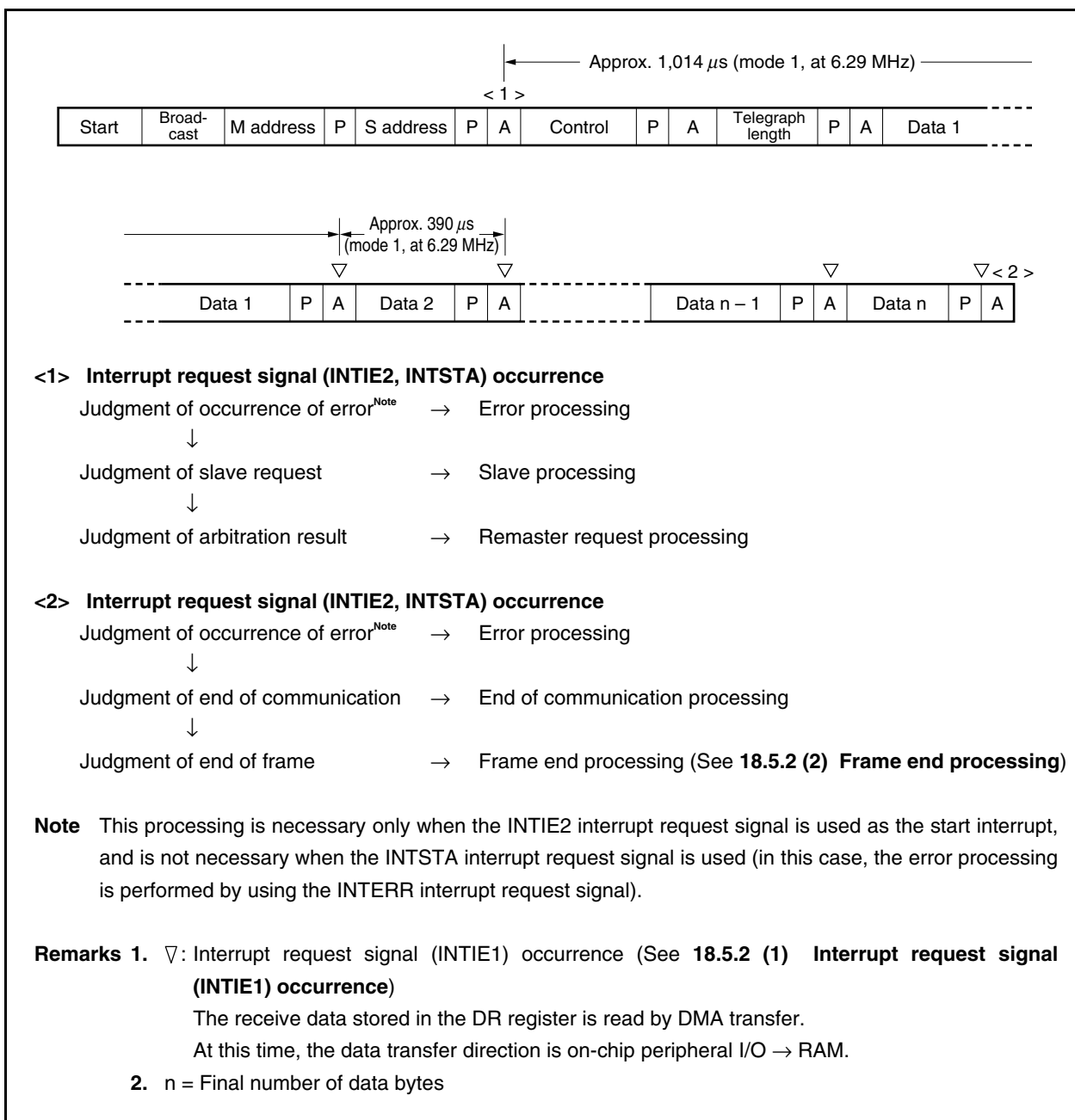
Figure 18-27. Master Reception
