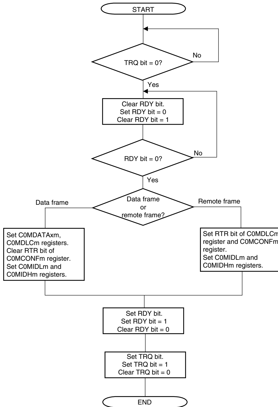
Figure 19-41. Message Transmit Processing
