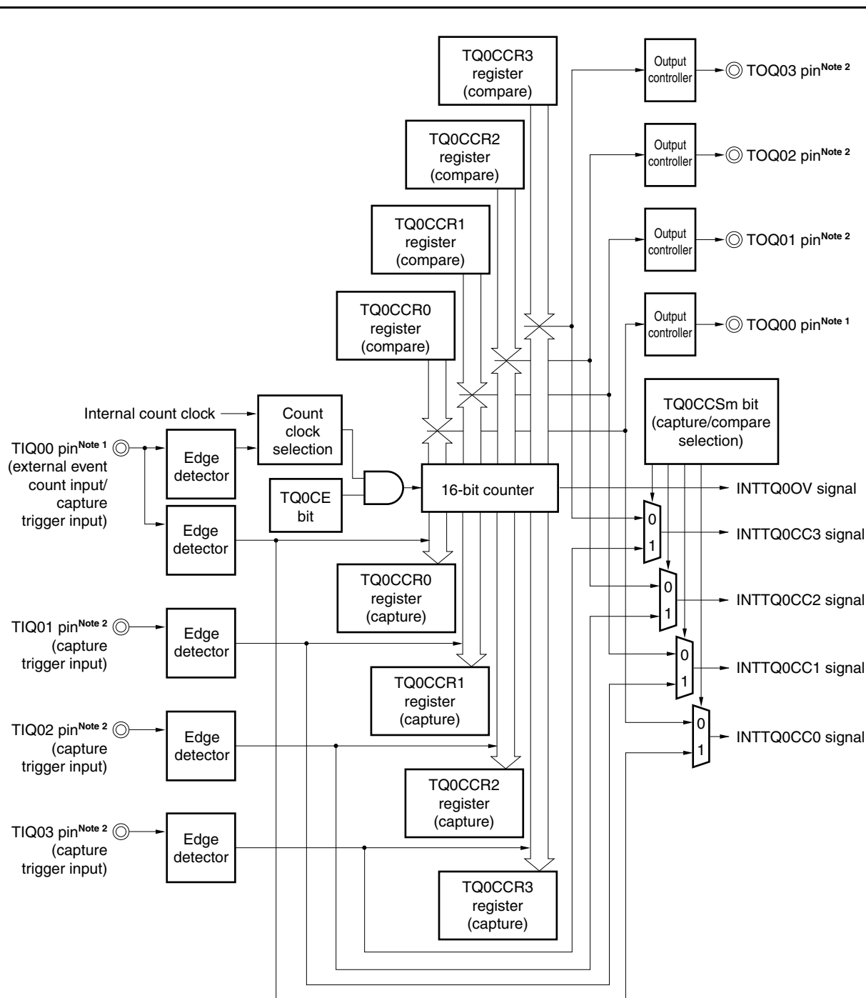
Figure 8-32. Configuration in Free-Running Timer Mode
