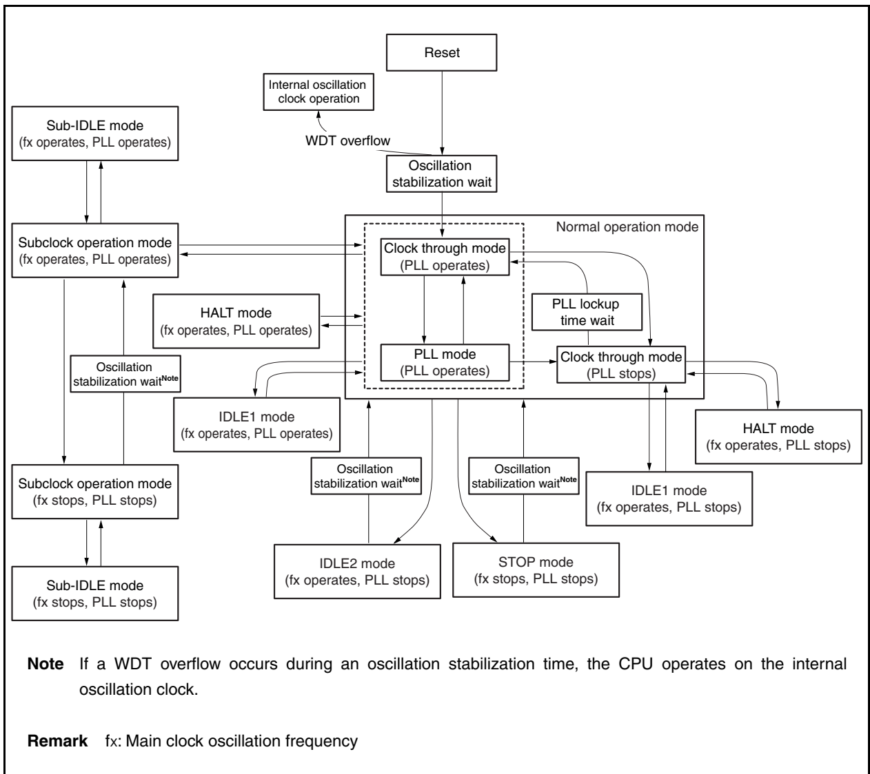
Figure 24-1. Status Transition
