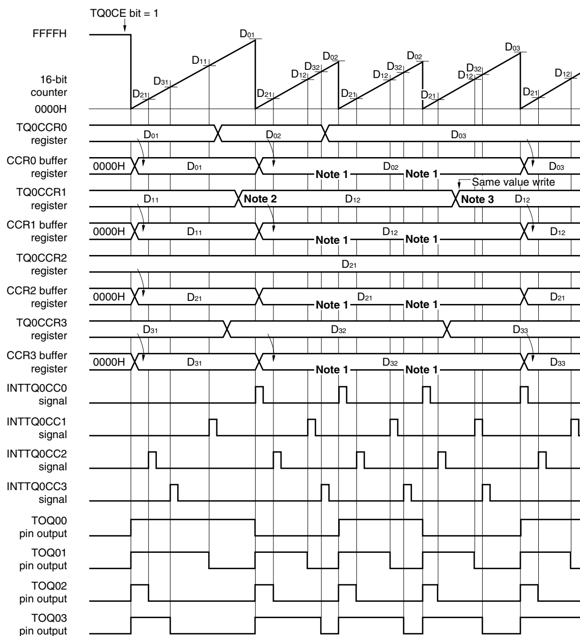
Figure 8-5. Timing of Batch Write
