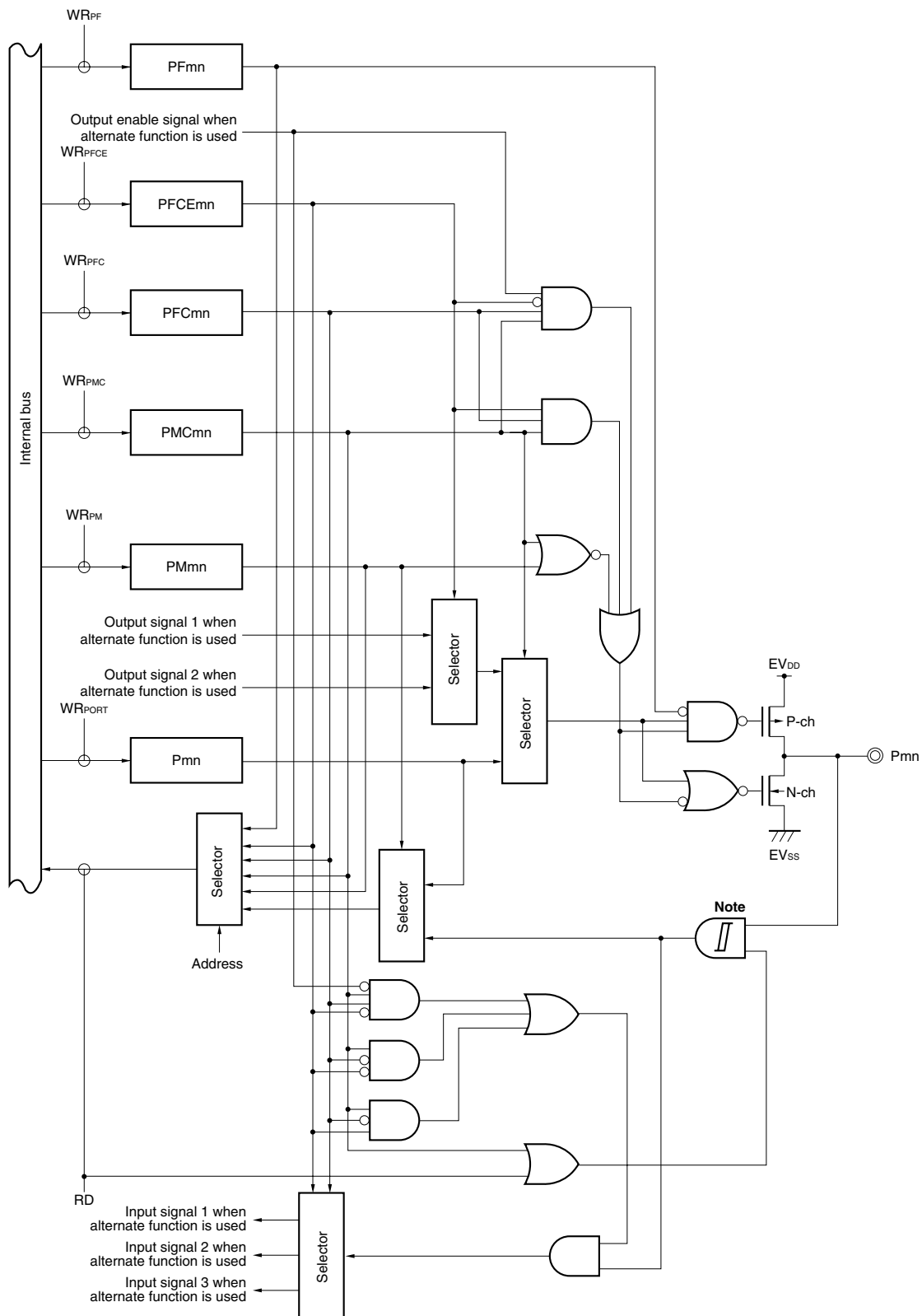
Figure 4-20. Block Diagram of Type U-1
