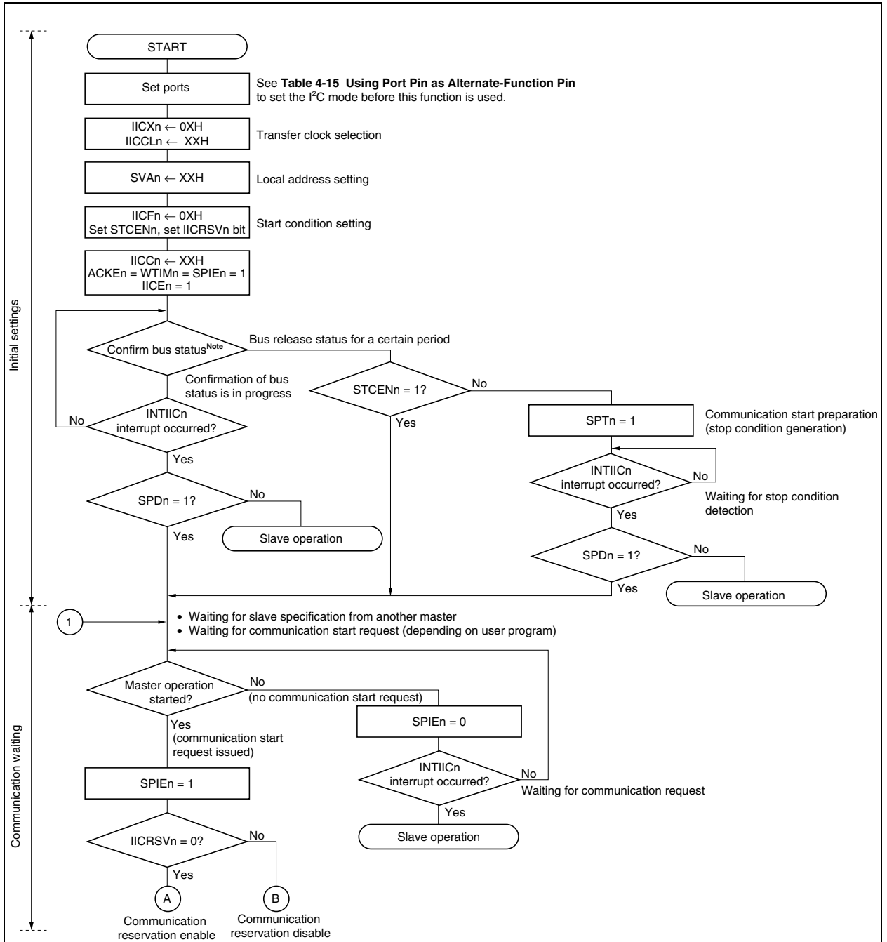
Figure 17-19. Master Operation in Multimaster System (1/3)
