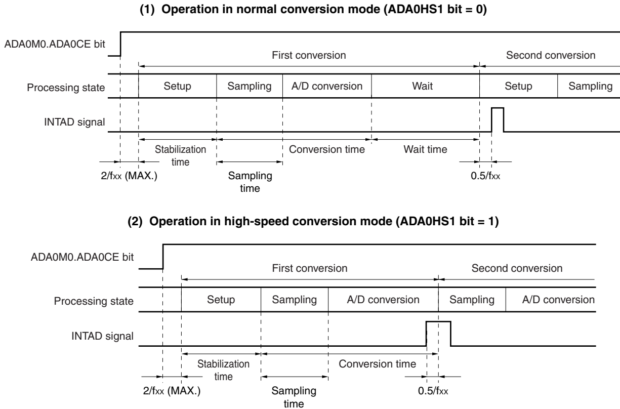
Figure 13-3. Conversion Operation Timing (Continuous Conversion)
