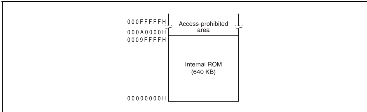
Figure 3-7. Internal ROM Area (640 KB)
