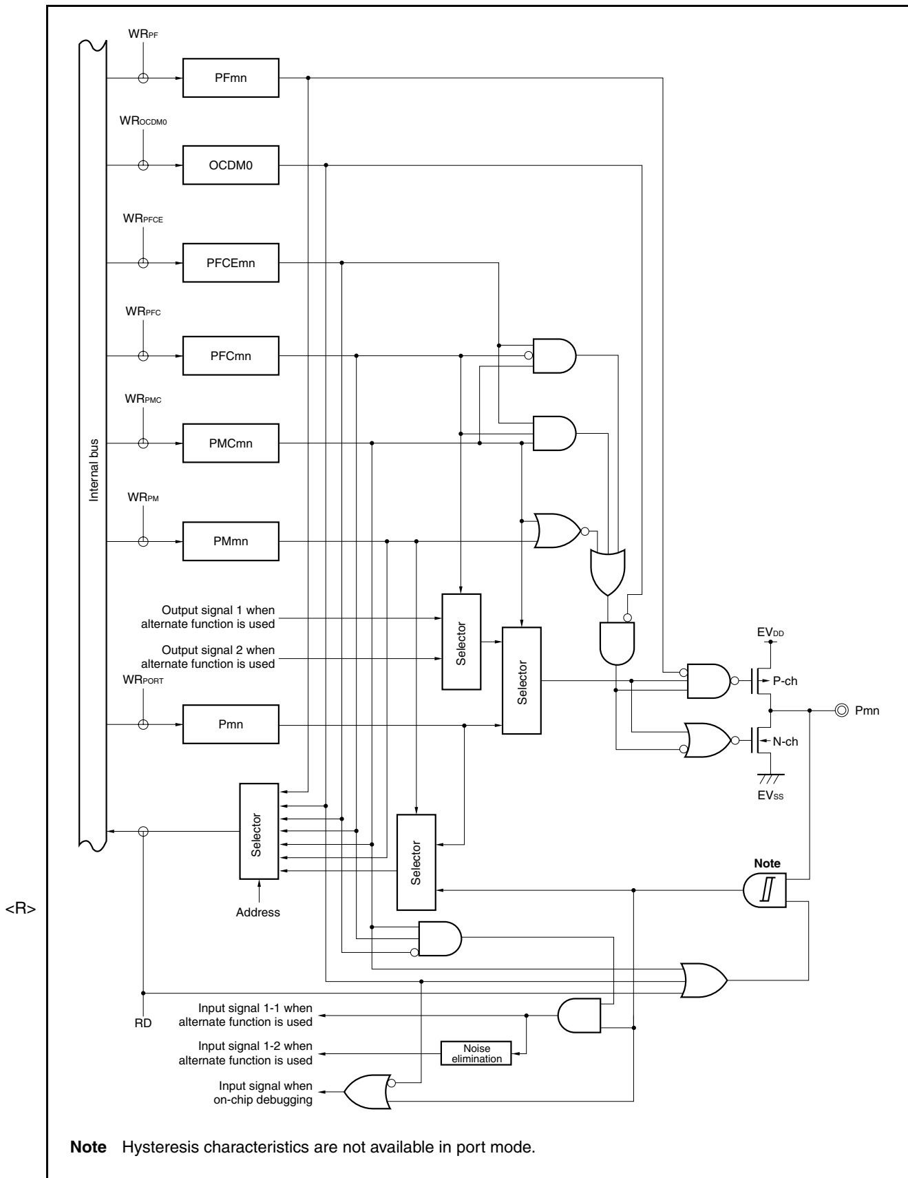
Figure 4-22. Block Diagram of Type U-6
