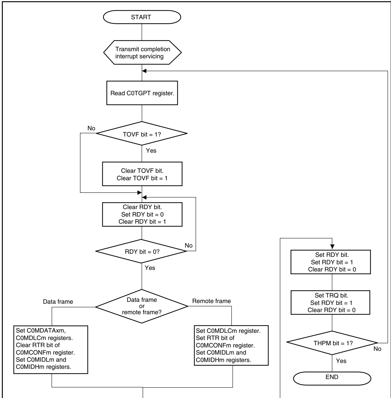
Figure 19-44. Transmission via Interrupt (Using C0TGPT Register)
