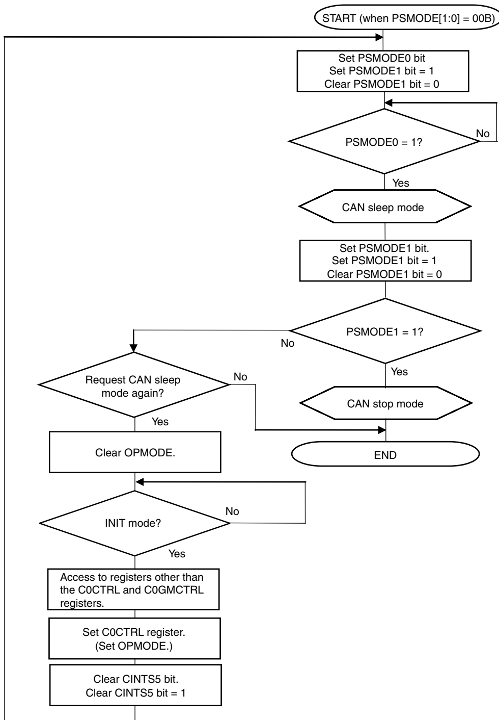
Figure 19-52. Setting CAN Sleep Mode/Stop Mode
