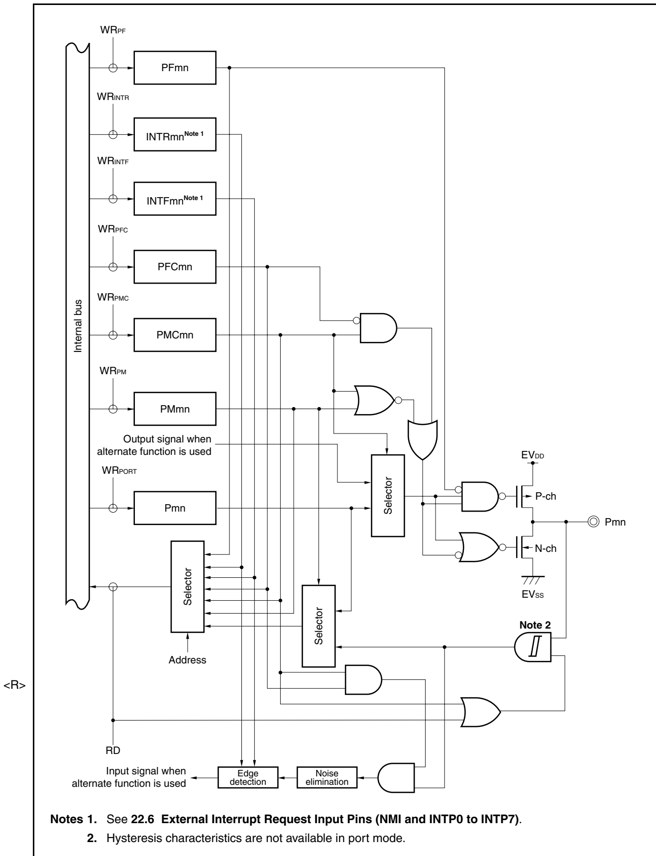
Figure 4-18. Block Diagram of Type N-2
