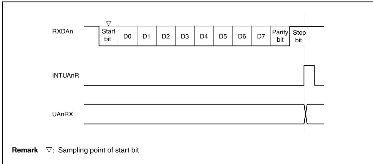
Figure 15-13. UART Reception
