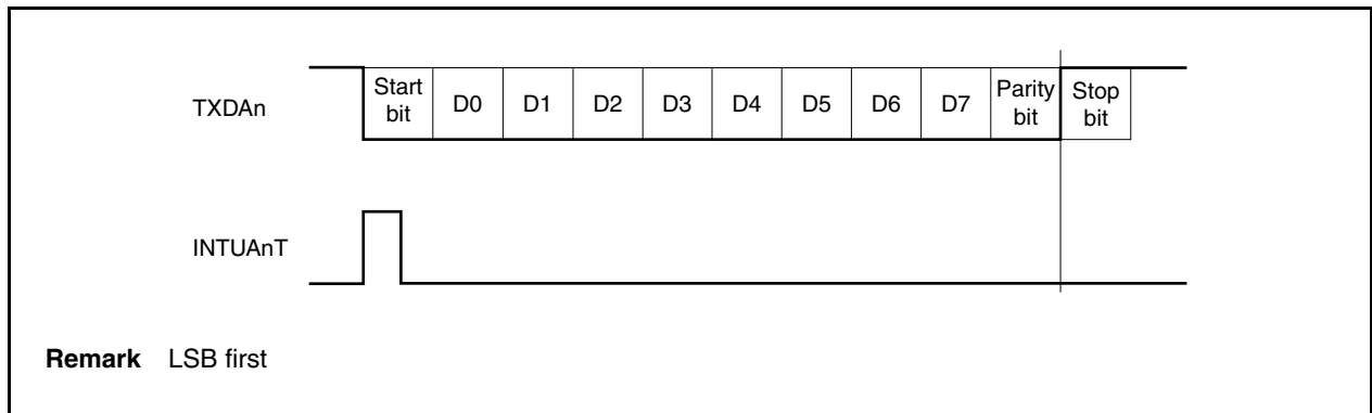
Figure 15-10. UART Transmission
