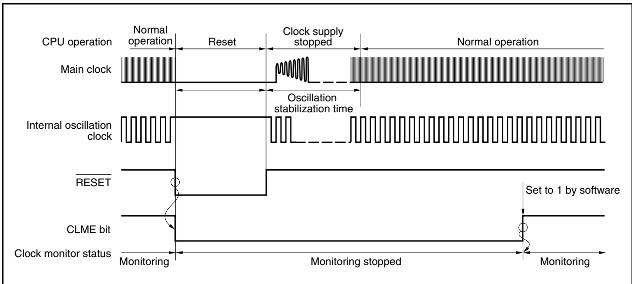
Figure 26-3. Clock Monitor Status After \overline{\text{RESET}} Input (CLM.CLME bit = 1 is set after \overline{\text{RESET}} input and at the end of main clock oscillation stabilization time)
