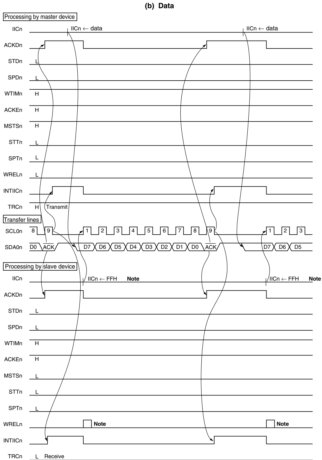
Figure 17-23. Example of Master to Slave Communication (When 9-Clock Wait Is Selected for Both Master and Slave) (2/3)
