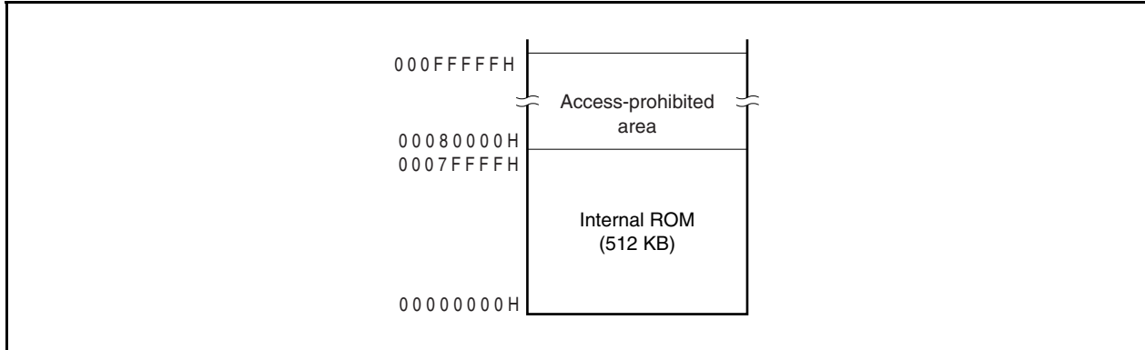
Figure 3-6. Internal ROM Area (512 KB)
