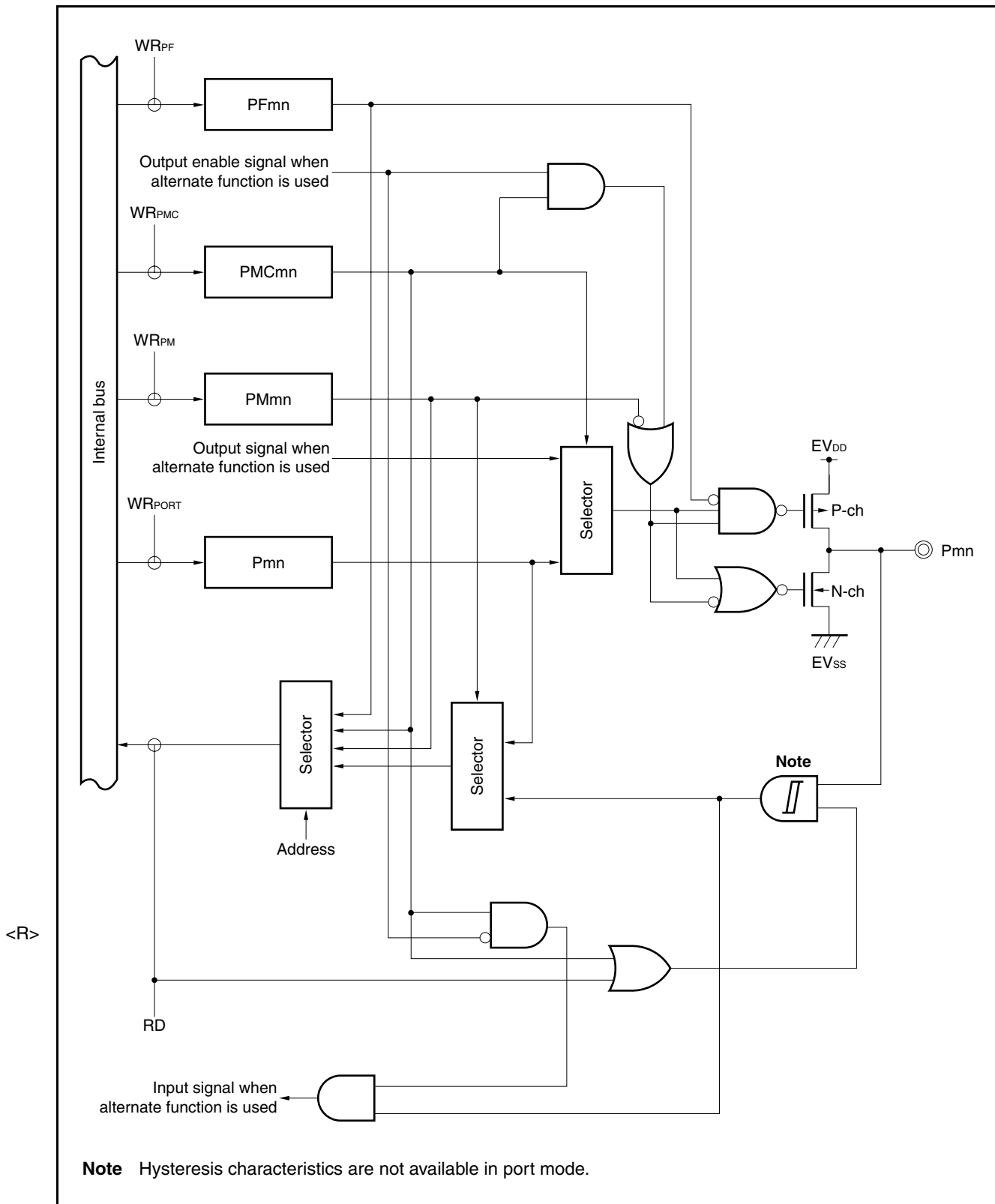
Figure 4-8. Block Diagram of Type E-3
