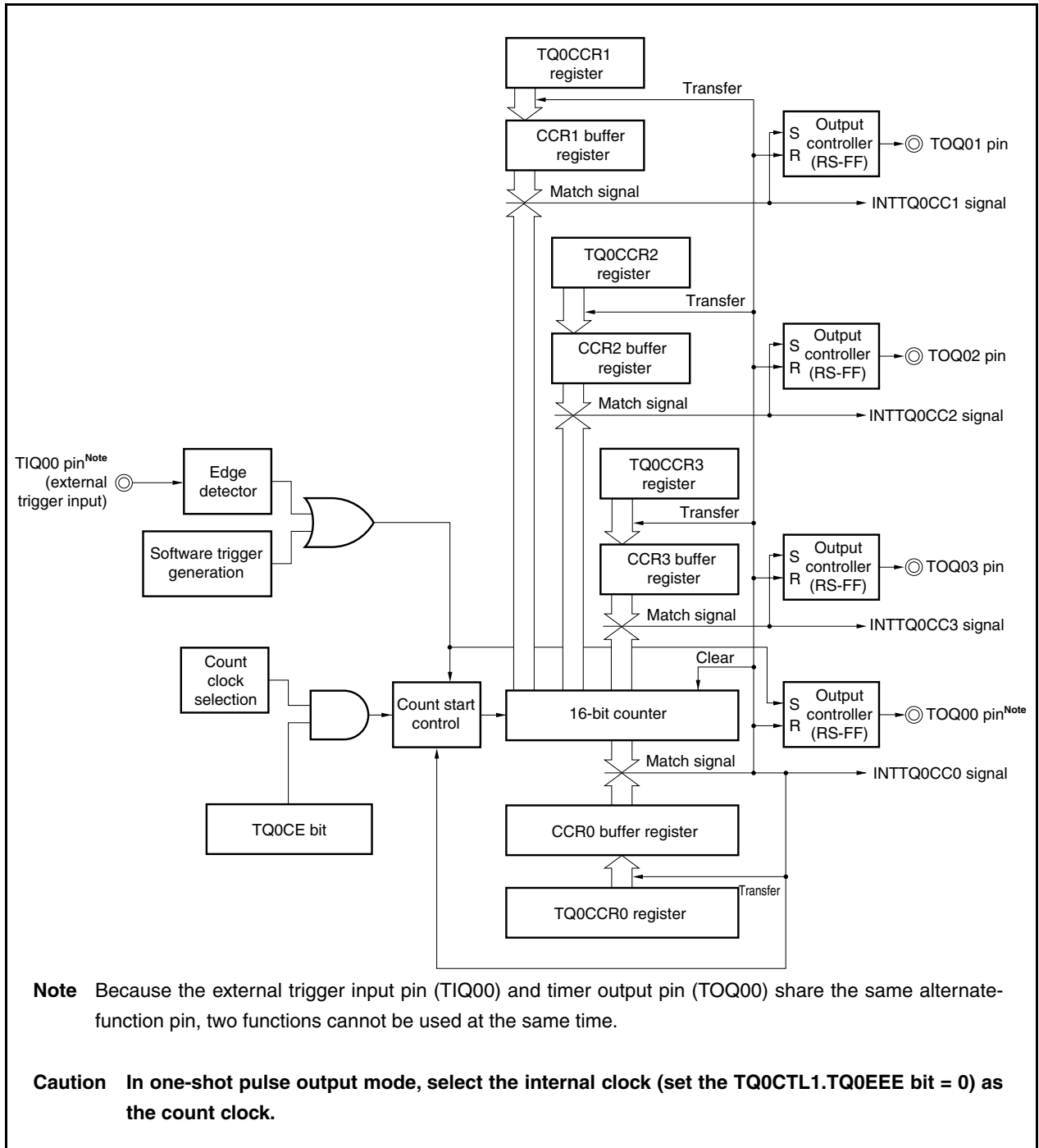
Figure 8-24. Configuration in One-Shot Pulse Output Mode
