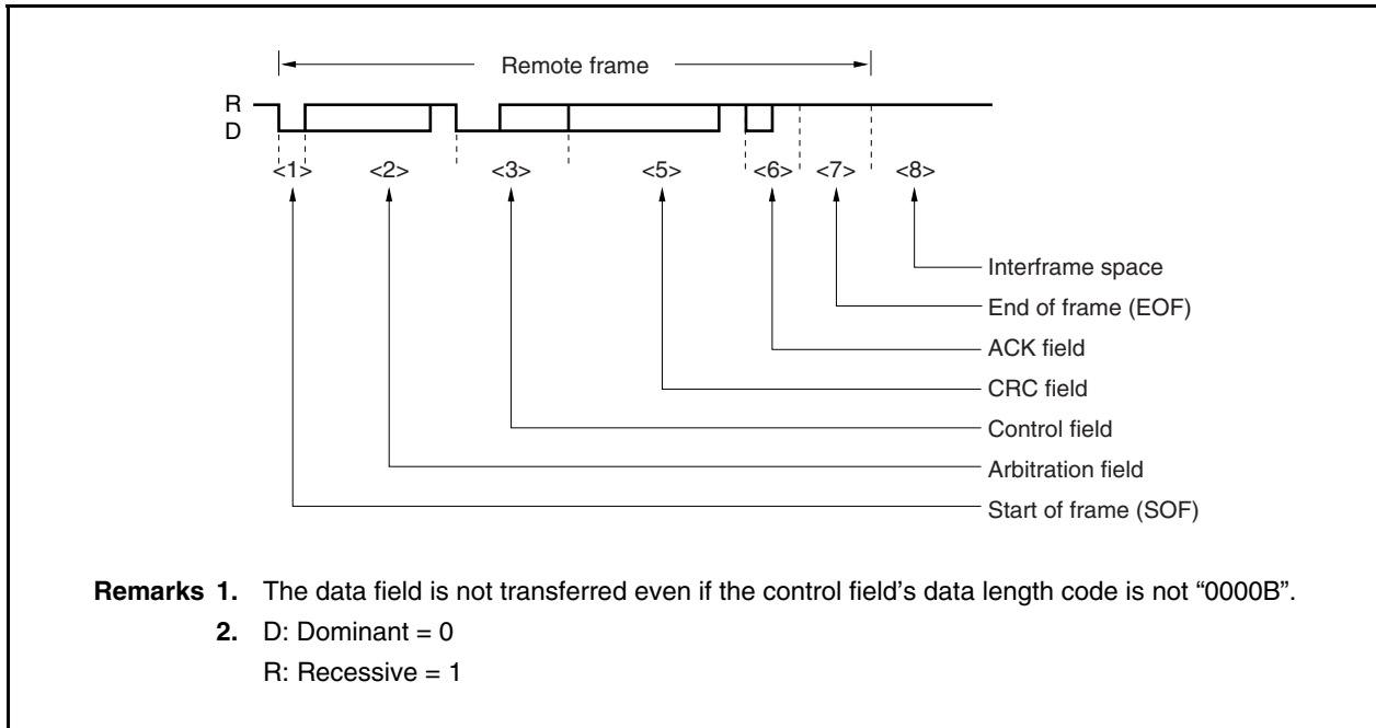
Figure 19-4. Remote Frame
