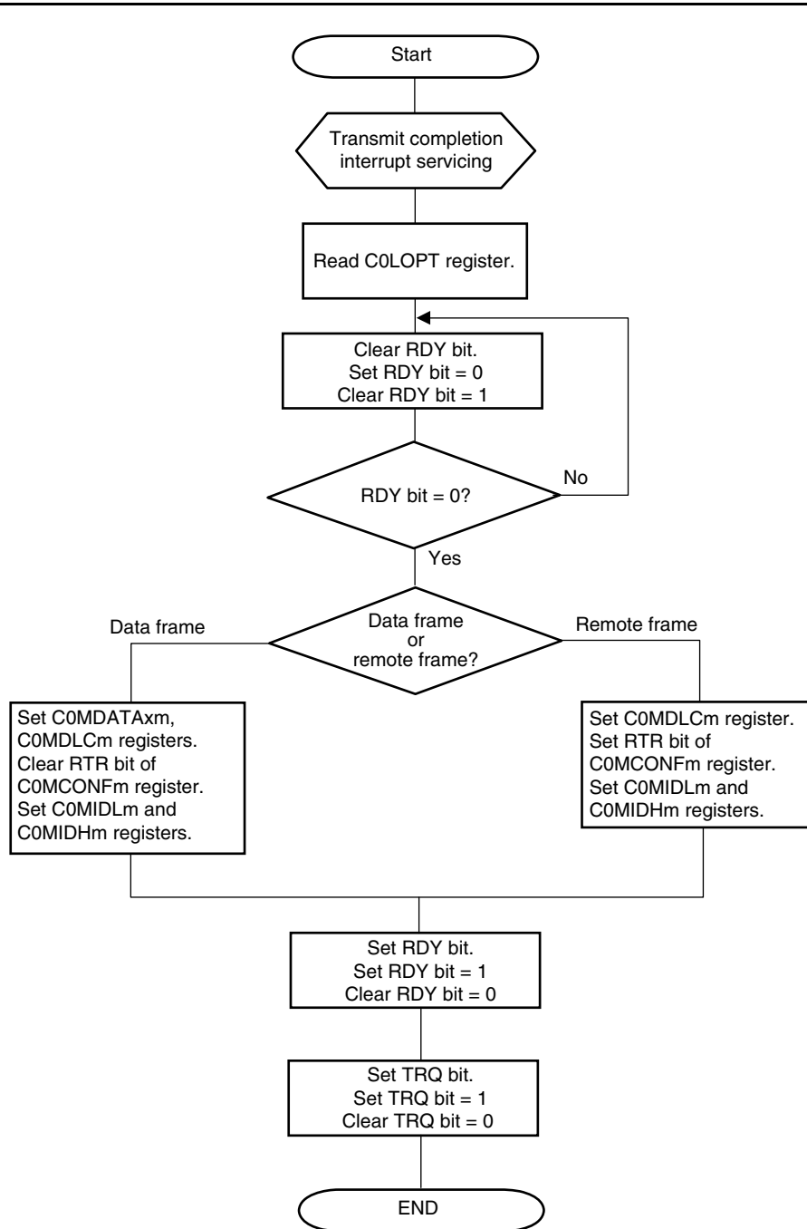
Figure 19-43. Transmission via Interrupt (Using C0LOPT register)
