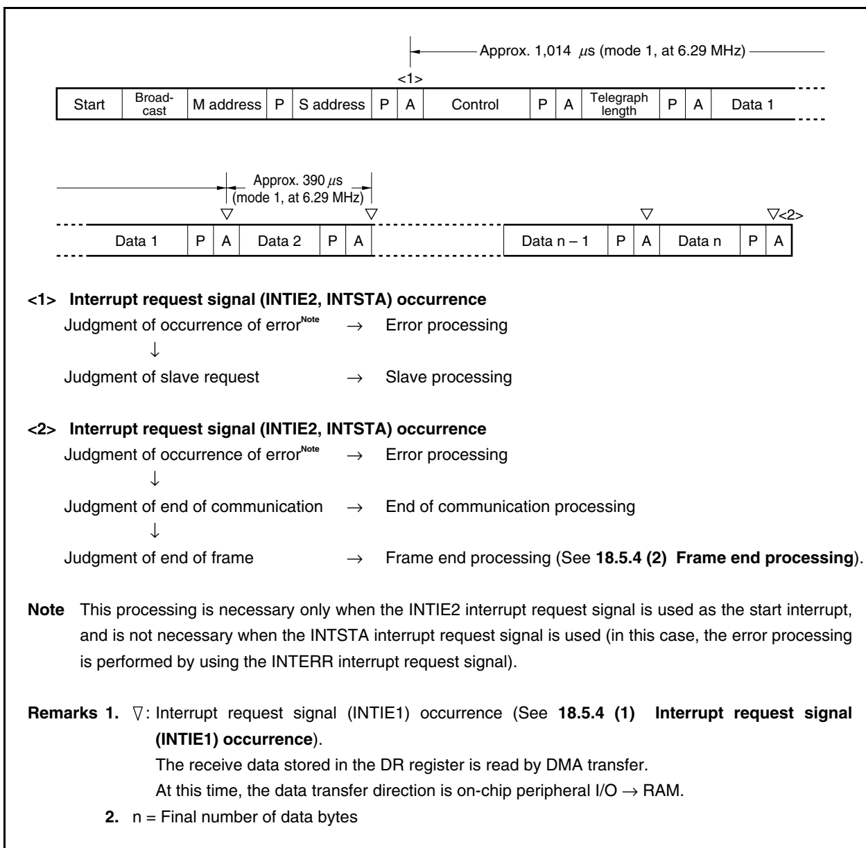
Figure 18-29. Slave Reception
