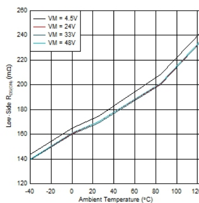
Figure 6-6. Low-Side R_{DS(ON)} over Temperature
