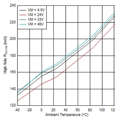
Figure 6-8. High-Side R_{DS(ON)} over Temperature
