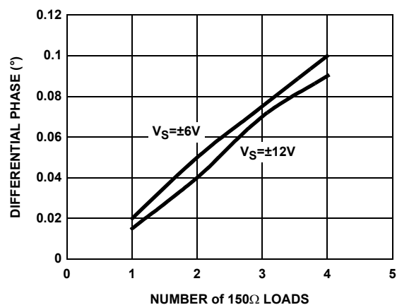
FIGURE 18. DIFFERENTIAL PHASE
