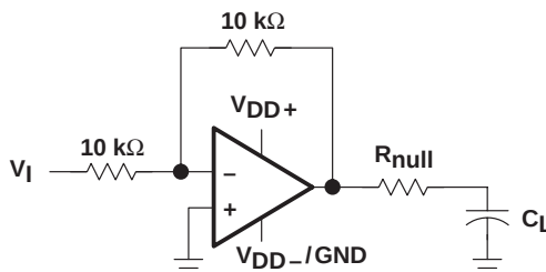
Figure 53. Series-Resistance Circuit
