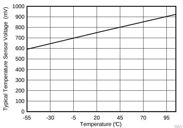
Figure 4-16. Typical Temperature Sensor Voltage
