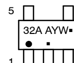
TSOP-5 (SOT23-5) SN SUFFIX CASE 483
